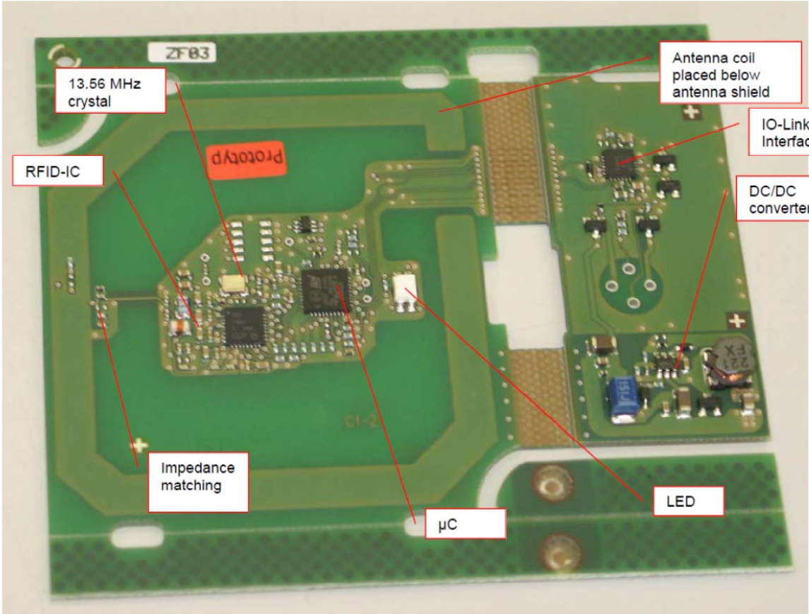
View on reader PCB (flat, prior to mounting into housing)
