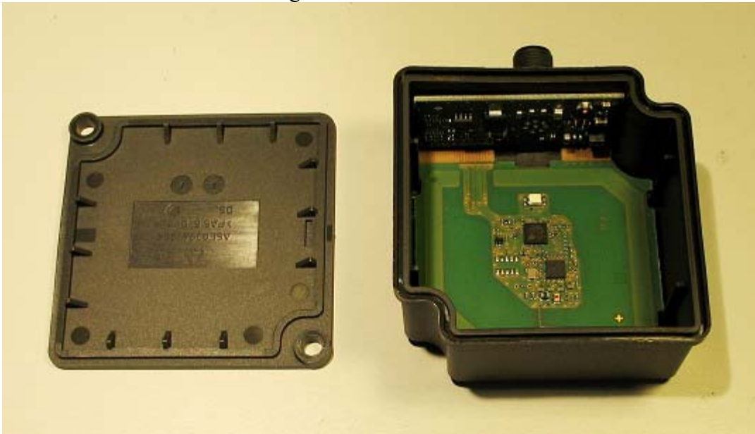
Reader-PCB in RF260R-housing
