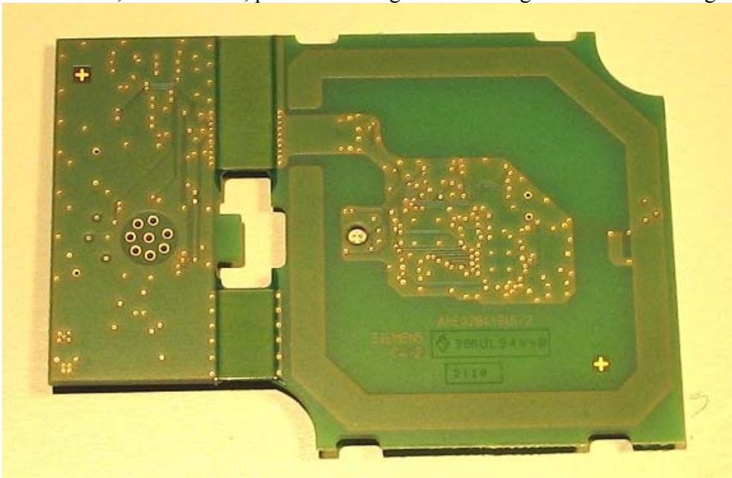
Reader-PCB, bottom-view, prior to bending and mounting in RF260R-housing
