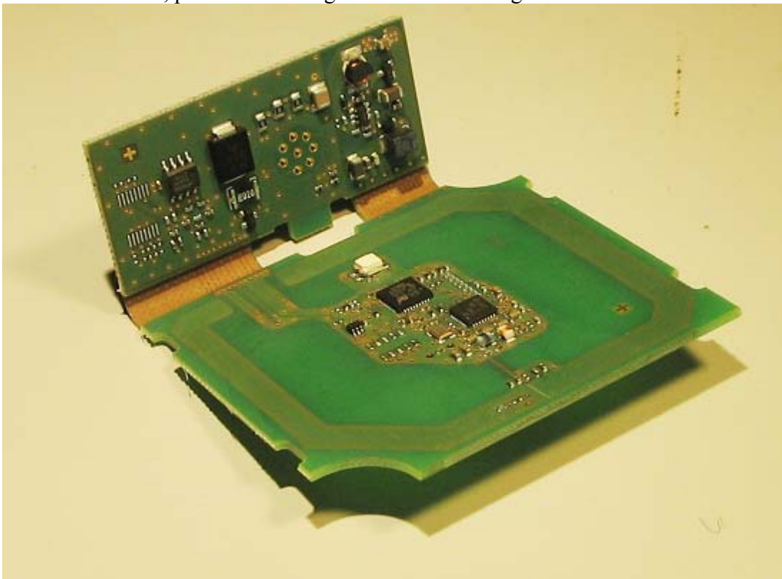
Reader-PCB bent, prior to mounting in RF260R-housing
