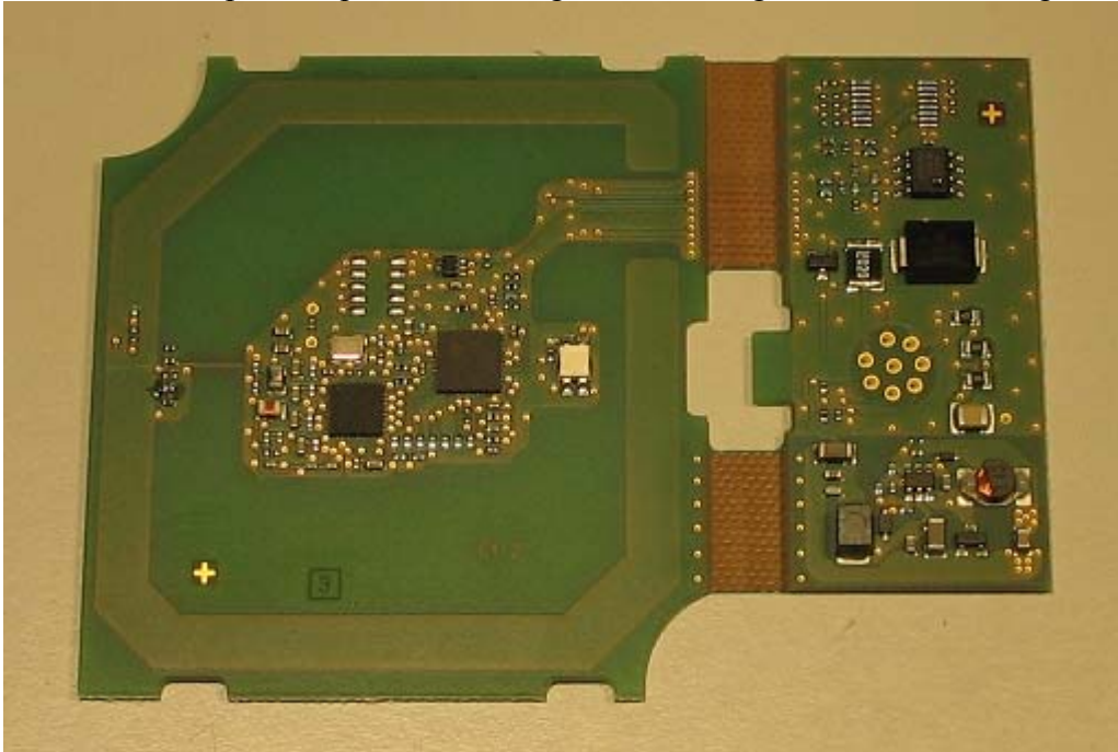
Reader-PCB, top-view, prior to bending and mounting in RF260R-housing
