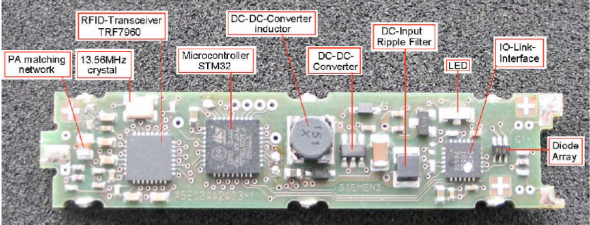
RF220R-IO-Link-Main PCB upper (top) side – close up
