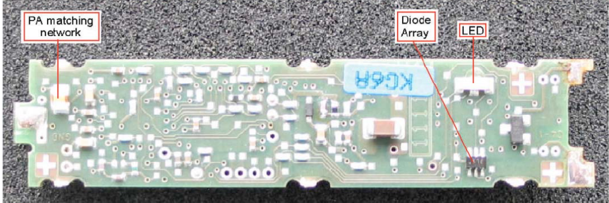
RF220R-IO-Link-Main PCB bottom side – close up
