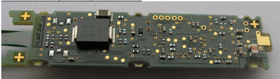
RF220R Main PCB, back side, without antenna
