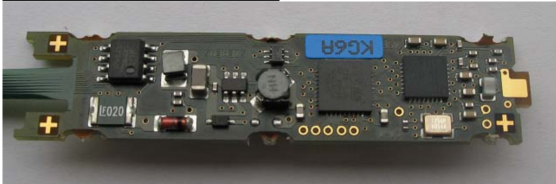
RF220R Main PCB, front side, without antenna
