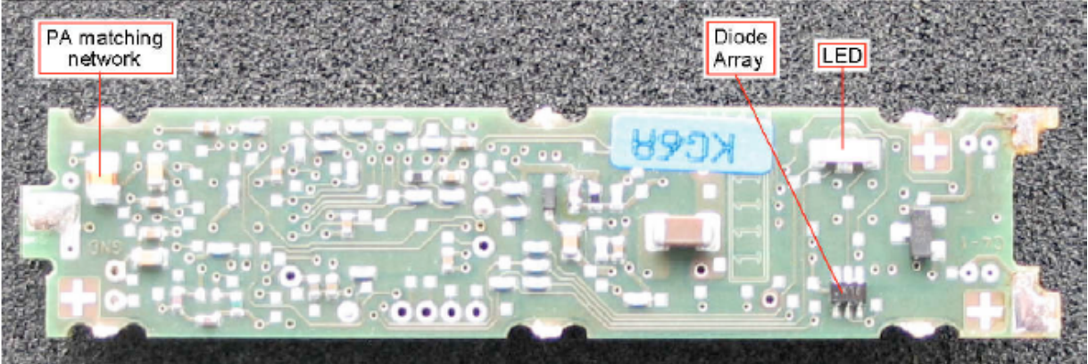
RF210R-IO-Link-Main PCB bottom side – close up
