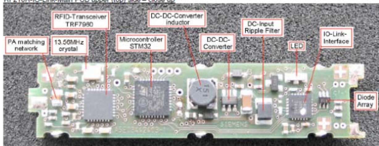
RF210R-IO-Link-Main PCB upper (top) side – close up
