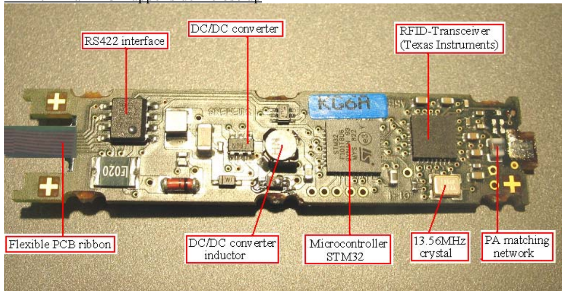
RF210R-main PCB upper side – close up
