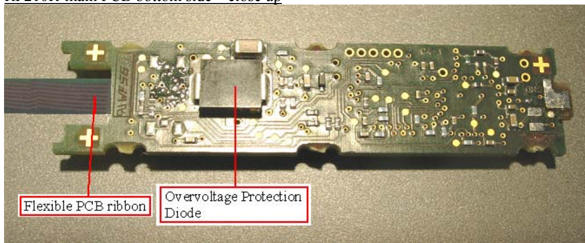
RF210R-main PCB bottom side – close up
