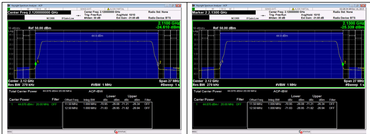
20 MHz Channel, QPSK
