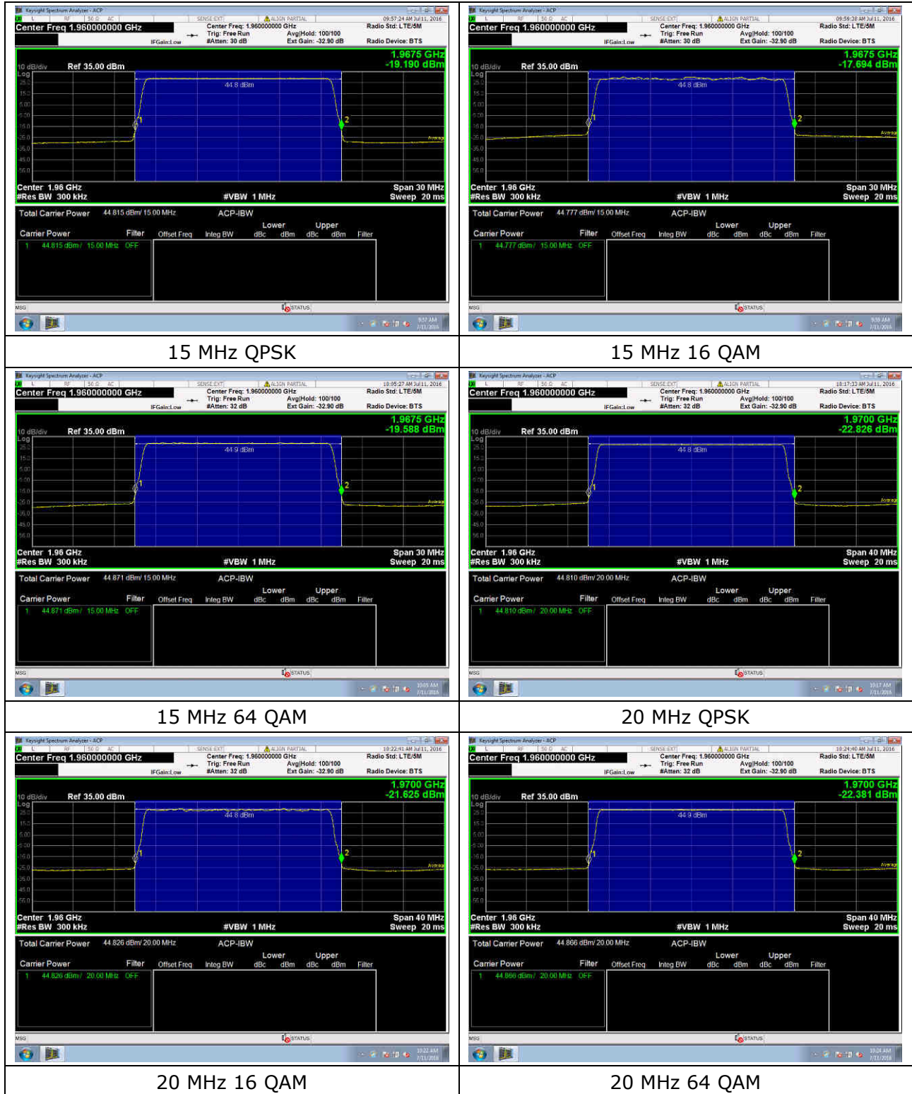
Figure 3: Transmit Power Plots
