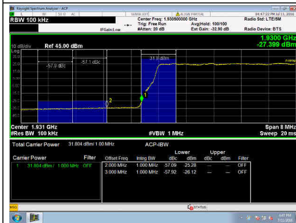
10 MHz 16QAM (bottom channel)
