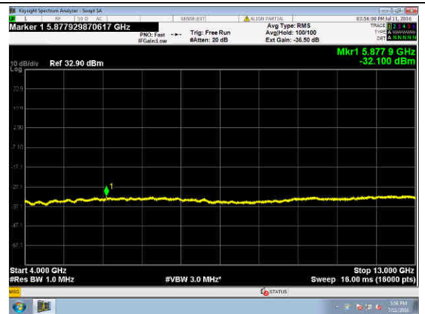
10 MHz 16QAM
