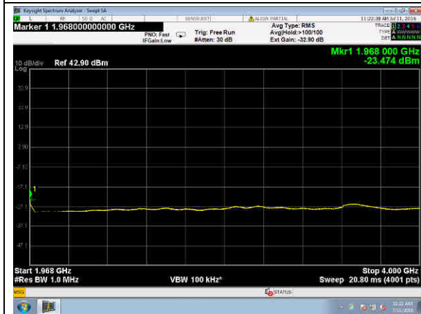
10 MHz 16QAM
