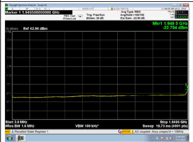
15 MHz 16QAM
