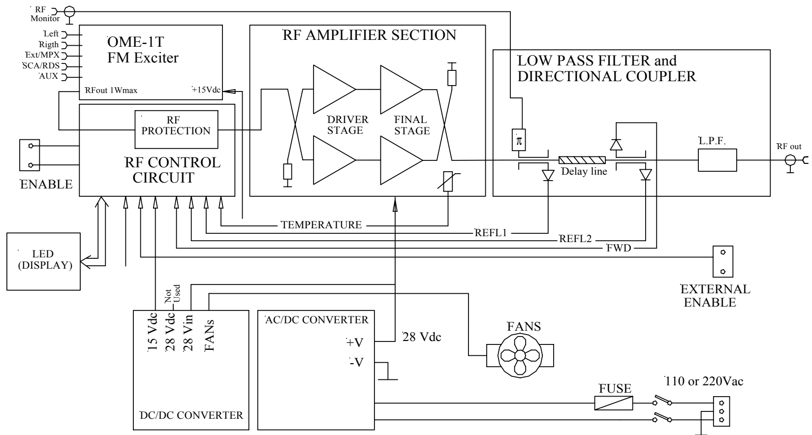
MT100 Block Diagram
