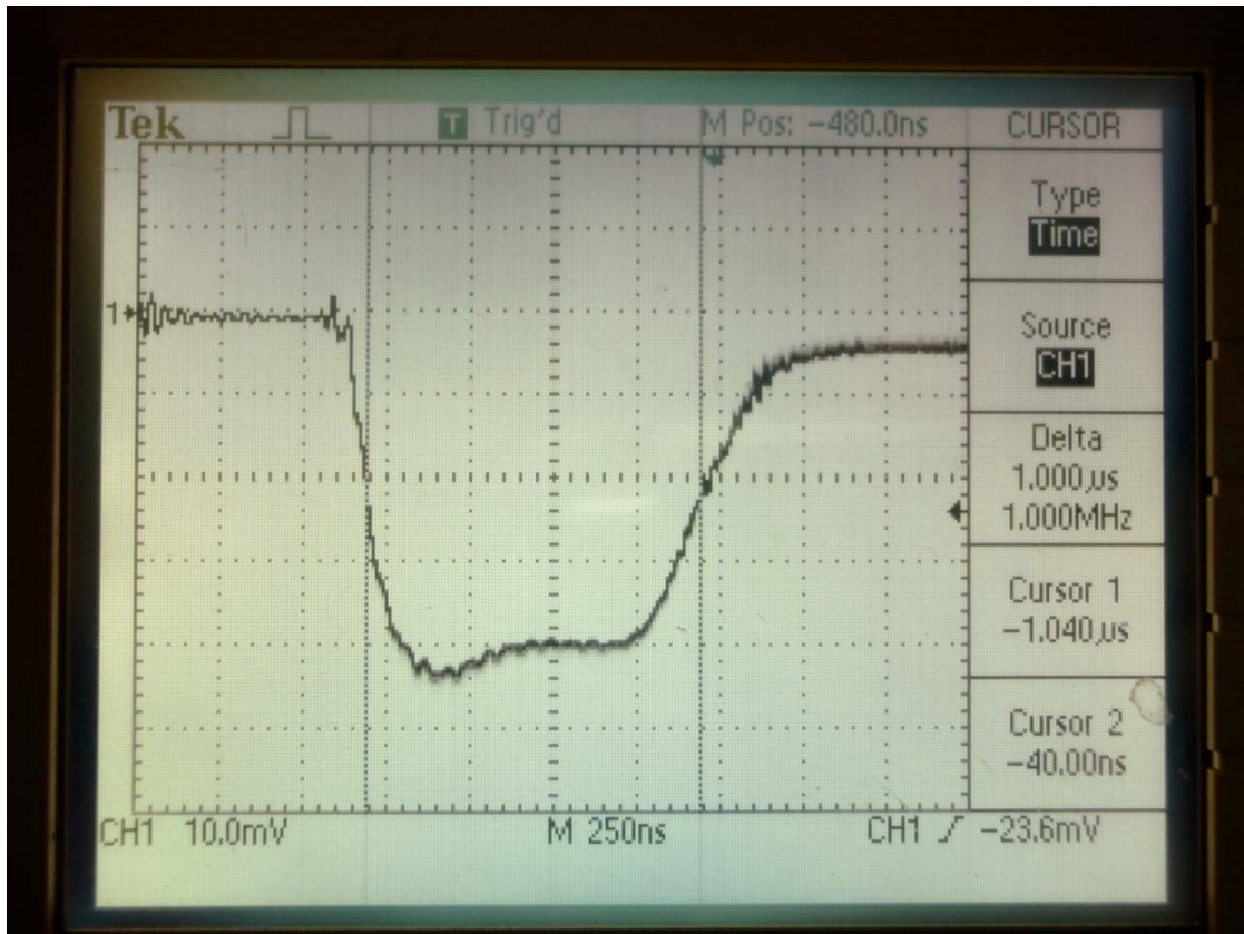
Plot #18: 1.0 μs Detected RF Pulse
