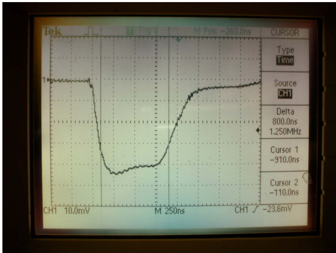
Plot #19: 0.8 \mu s Detected RF Pulse
