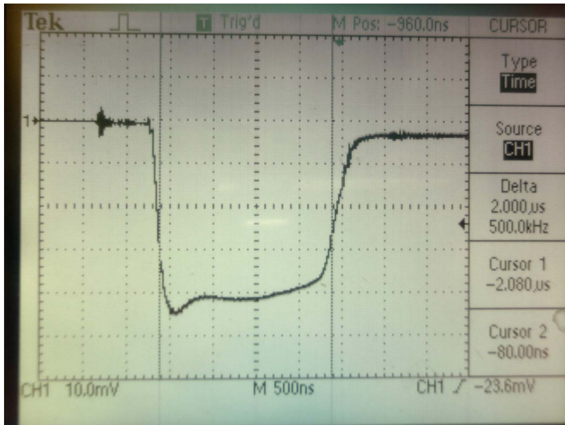
Plot #17: 2.0 \mu s Detected RF Pulse
