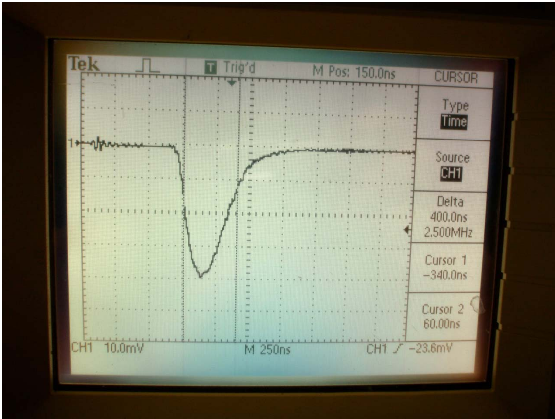
Plot #20: 0.4 \mu s Detected RF Pulse
