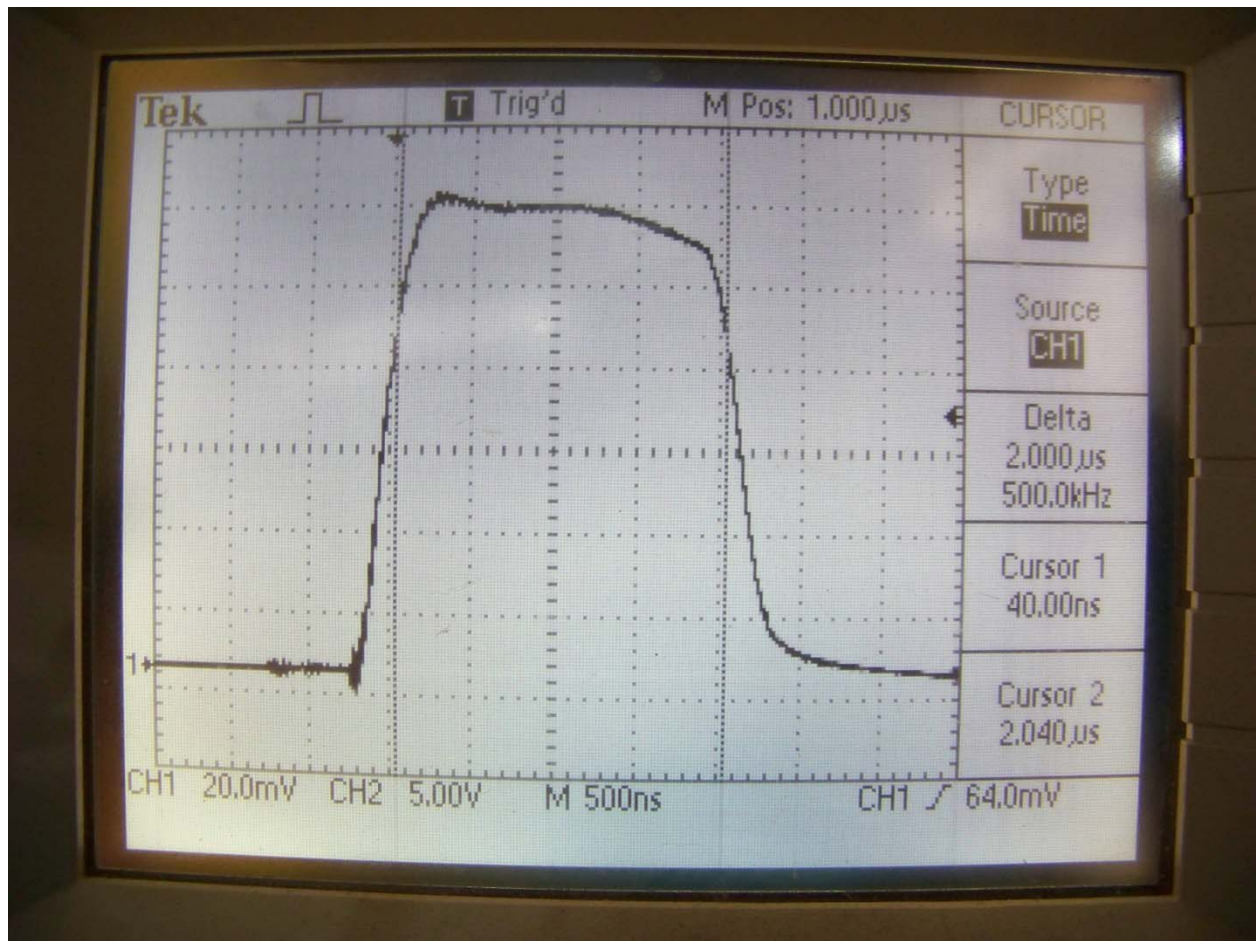
Plot #22: 2.0μs Detected RF Pulse
