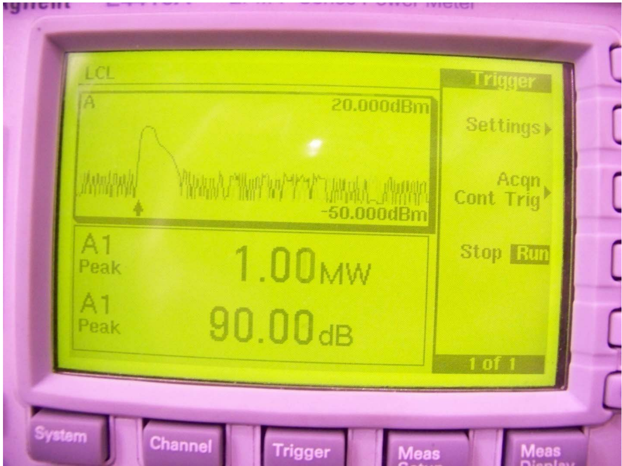
Plot #27: 0.8us RF Pulse, 81.2dBm attenuation correction
