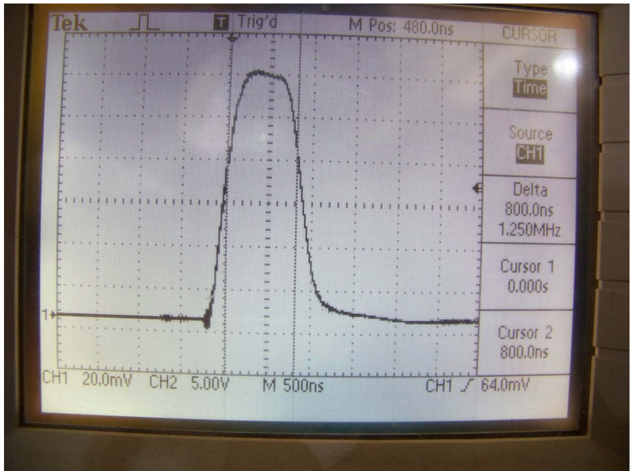
Plot #24: 0.8 \mu s Detected RF Pulse
