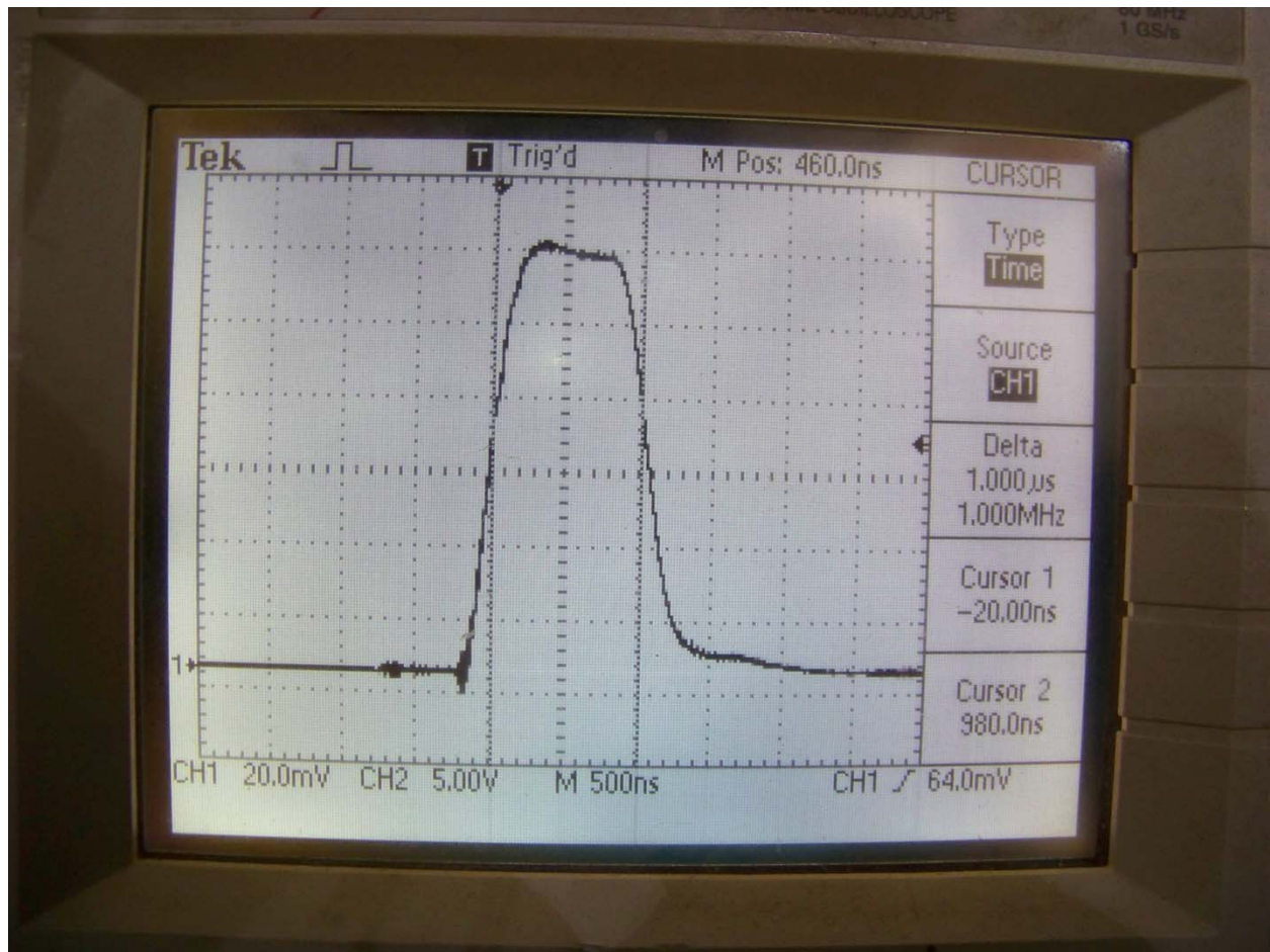
Plot #23: 1.0µs Detected RF Pulse
