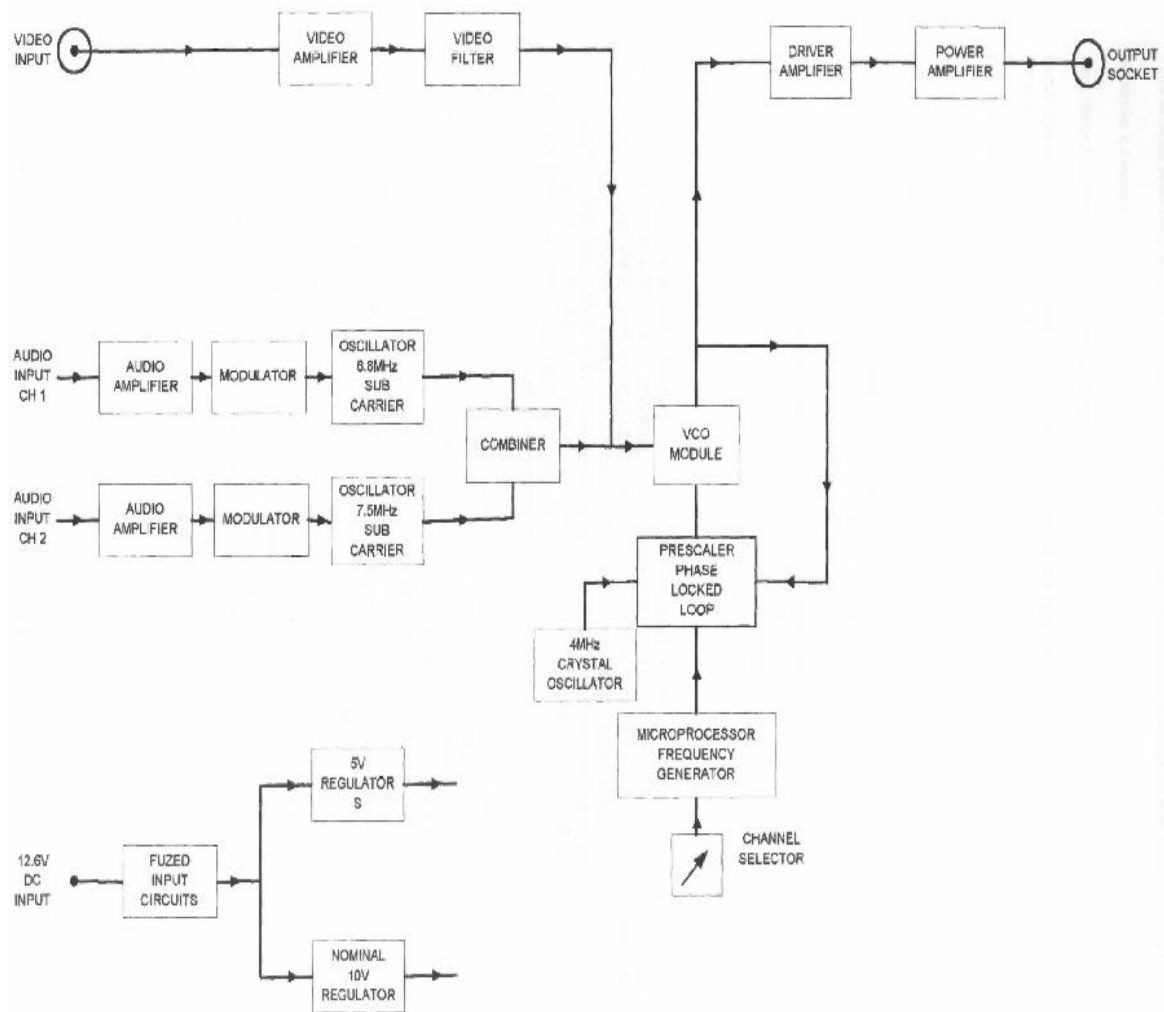
3. BLOCK DIAGRAM FOR VT240SC2D VIDEO TRANSMITTER
