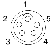
Figure iii : 5 Pin LEMO pin out orientation viewed from solder spill side
