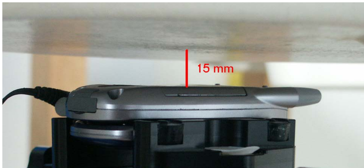
Fig. 30: Body worn configuration with headset and 1.5 cm distance(1 TX slot).
