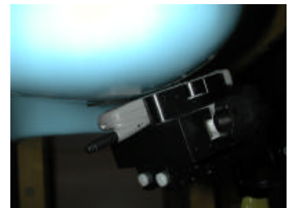
Figure 19. Head SAR Test Setup
