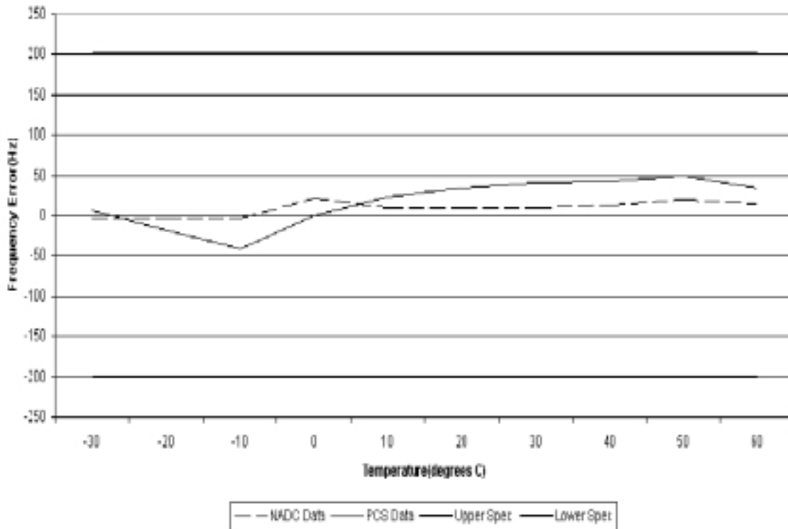
Frequency Stability Over Temperature - TDMA 800 & PCS
