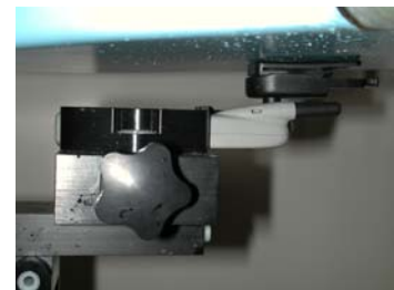
Figure 20. Body SAR Test Setup
