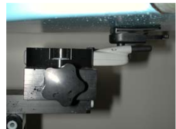
Figure 21. Body SAR Test Setup
