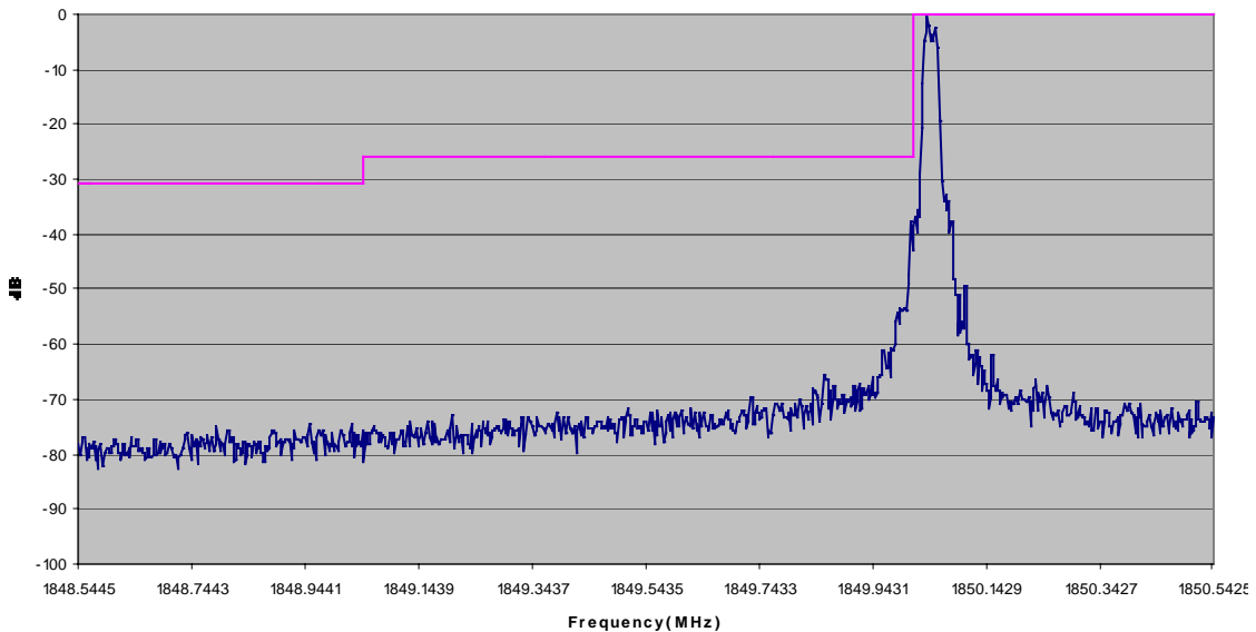
Out of Band Emissions - PCS Low Side < 1 MHz
