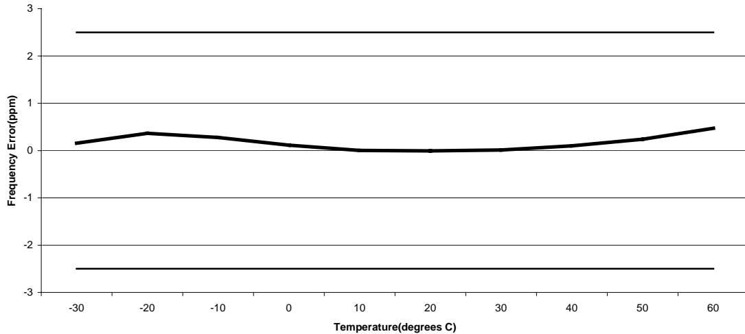
Frequency Stability Over Temperature - AMPS
