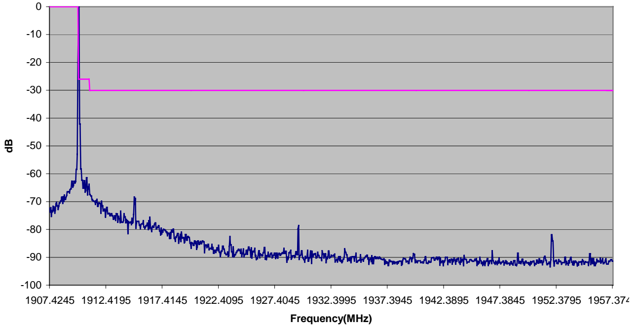
Out of Band Emissions - PCS High Side > 1 MHz
