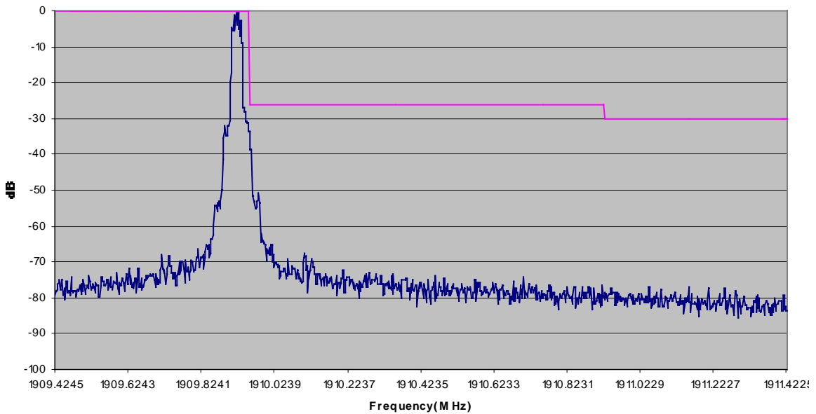
Out of Band Emissions - PCS High Side < 1 MHz
