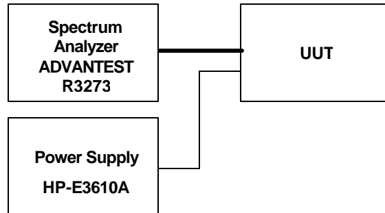
Test Setup for Conducted Spurious Emissions
