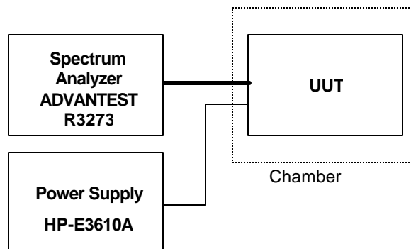
Test Setup for Frequency Stability
