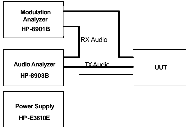
Test Setup for Audio Frequency Response
