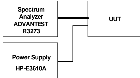
Test Setup for Occupied Band Width
