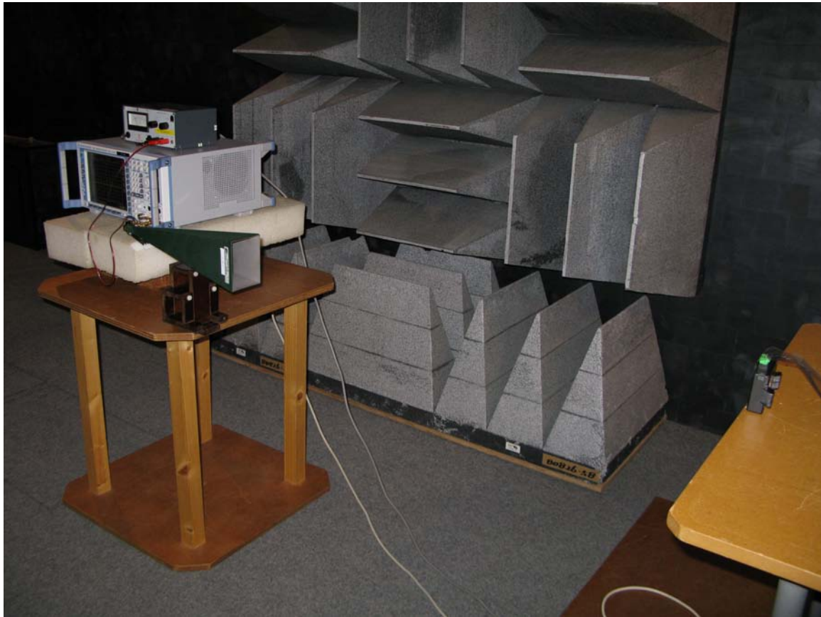
Photograph 3: radiated emissions test set up (18 - 26 GHz)
