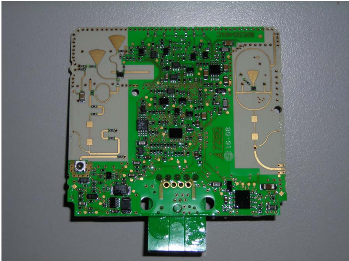
Photograph 3: PCB bottom view of MMS
