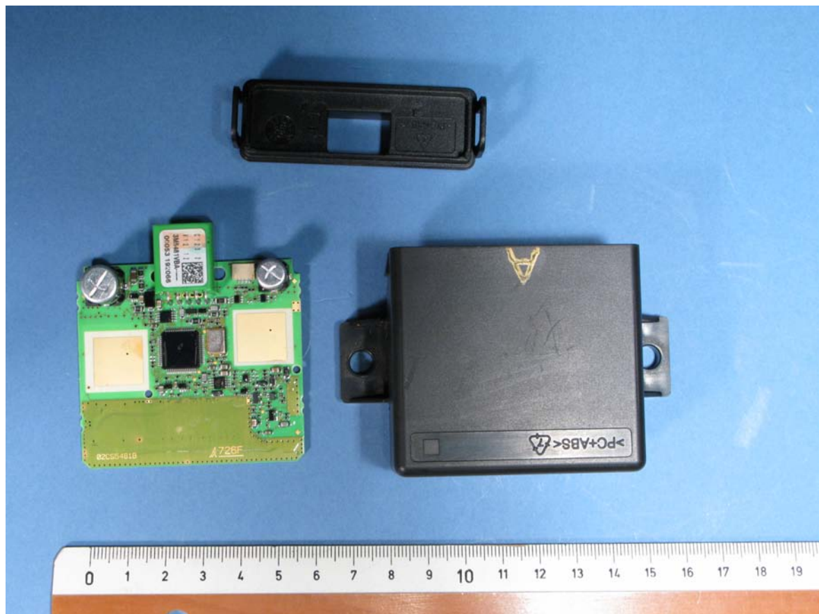
Photograph 1: exploded view of MMS
