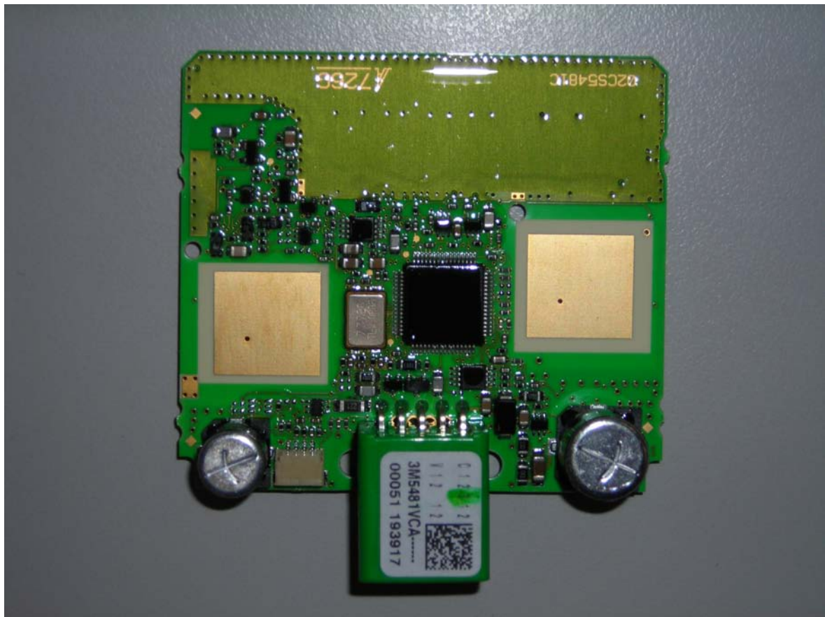
Photograph 2: PCB top view of MMS
