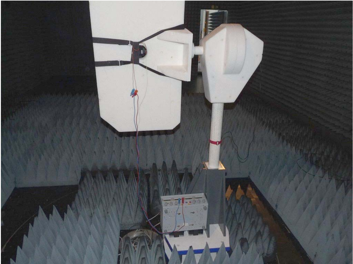
Photo 3: Test setup for radiated measurements (Enclosure, above 1 – 26.5 GHz)
