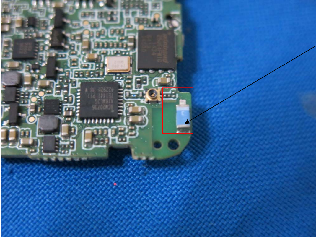
BT Antenna
