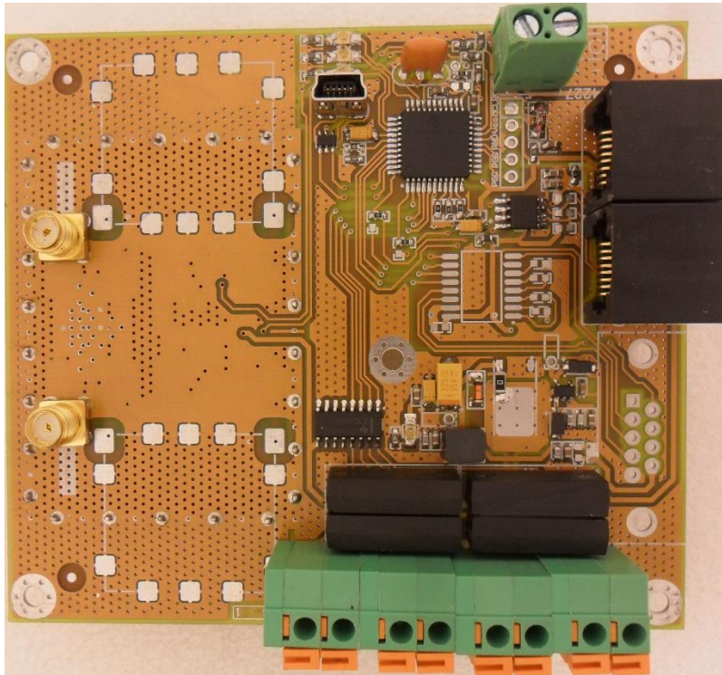
NFPA BOARD PCB – TOP
