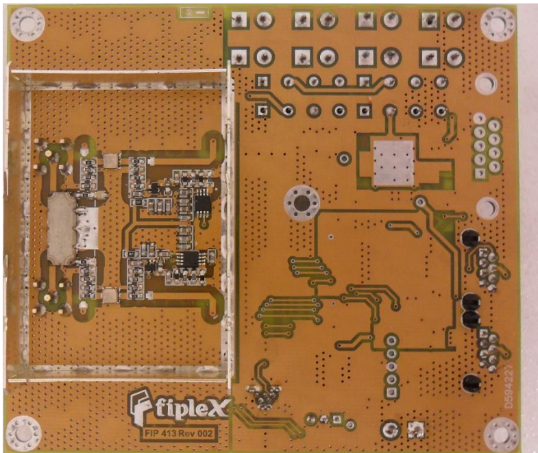
NFPA BOARD PCB - BOTTOM
