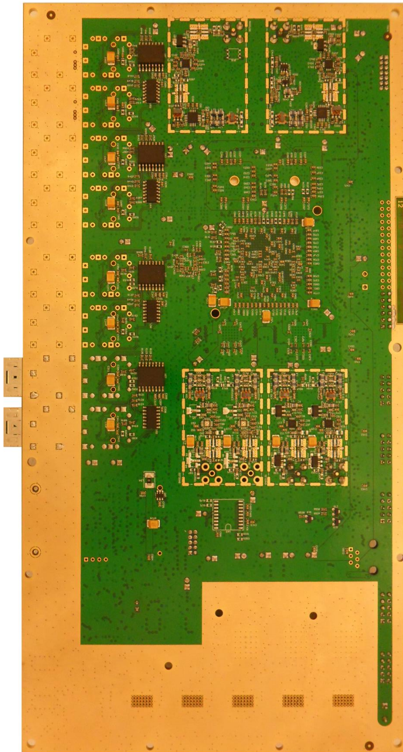
DIGITAL BOARD PCB – BOTTOM
