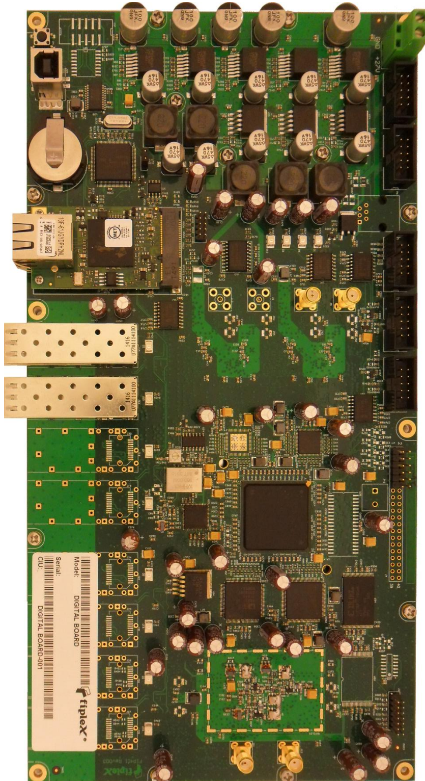
DIGITAL BOARD PCB - TOP
