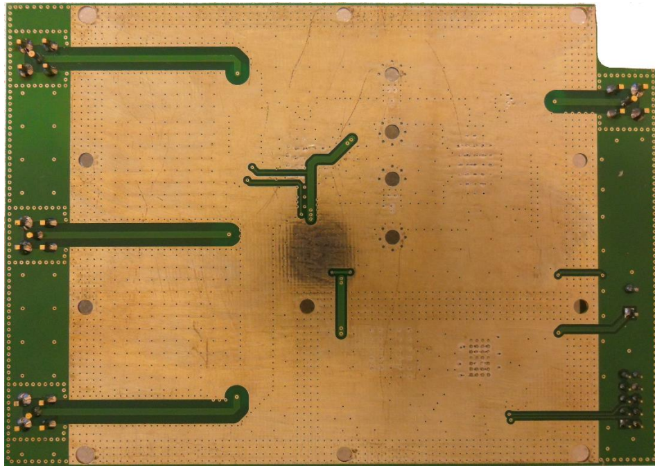
(PALP) LOW POWER AMPLIFIER PCB – BOTTOM
