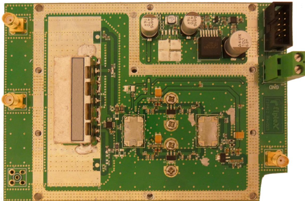
(PALP) LOW POWER AMPLIFIER PCB – TOP
