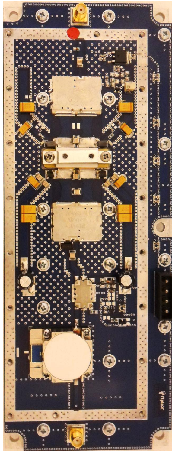
(PAHP) HIGH POWER AMPLIFIER PCB – TOP
