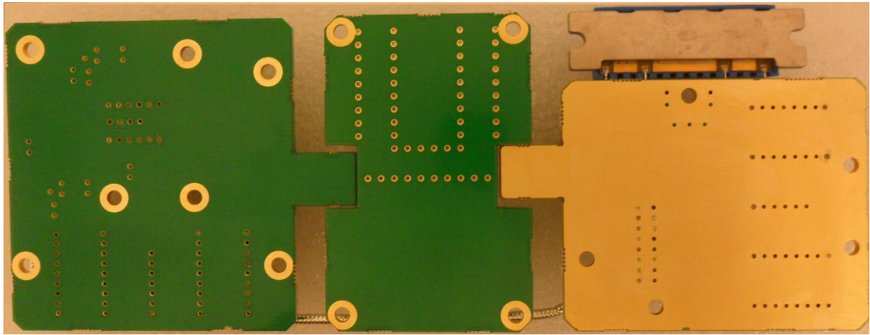
(PAMP) MEDIUM POWER AMPLIFIER PCB - BOTTOM
