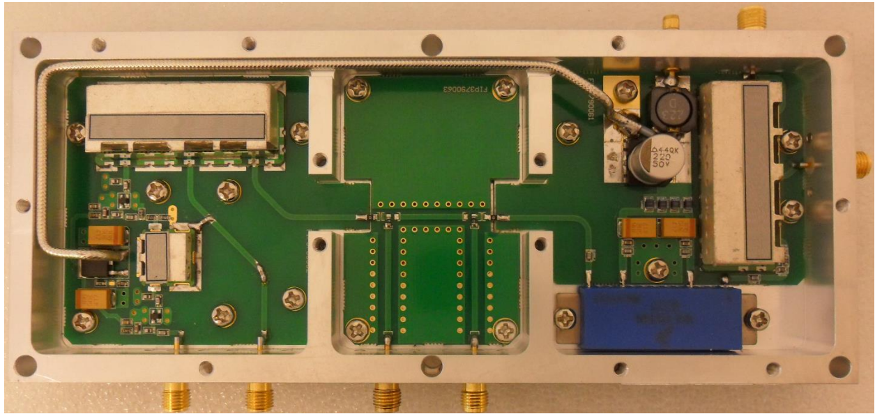
(PAMP) MEDIUM POWER AMPLIFIER BLOCK – TOP
