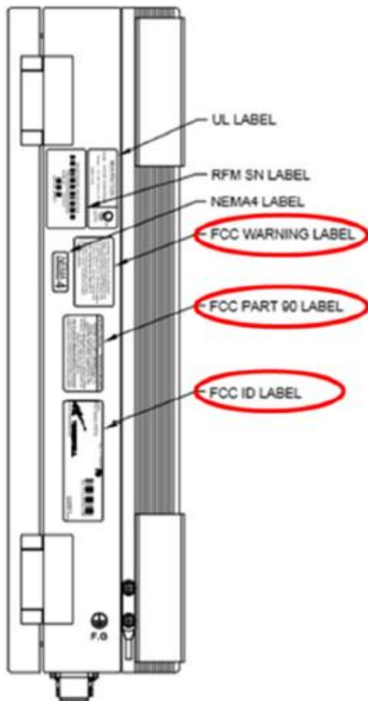
Right-Side View
