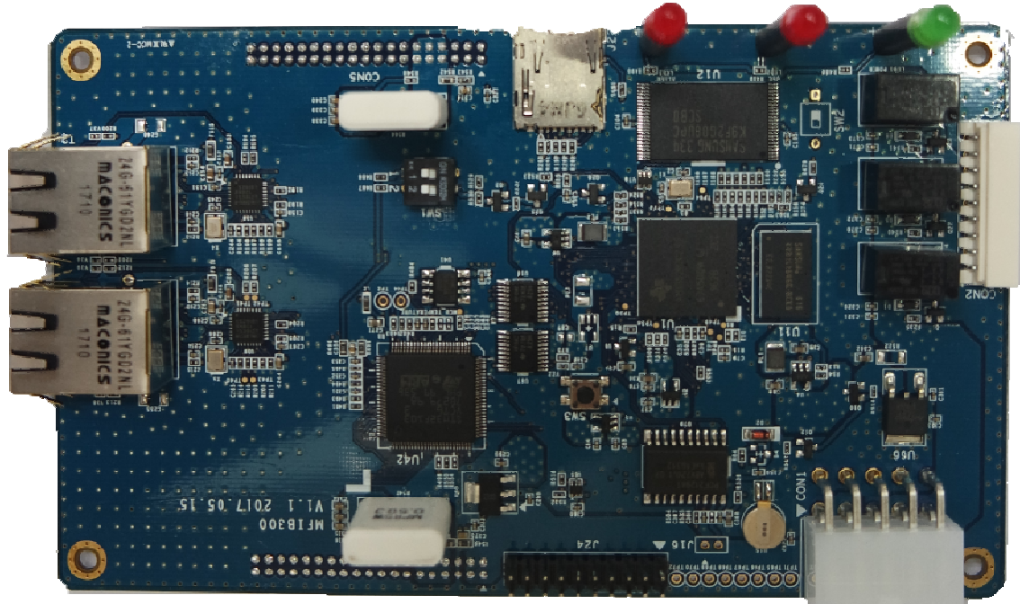
MFIB 300 (TOP)
