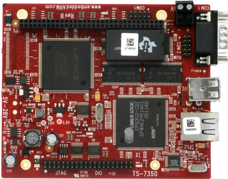
Single Board Computer Comp Side
