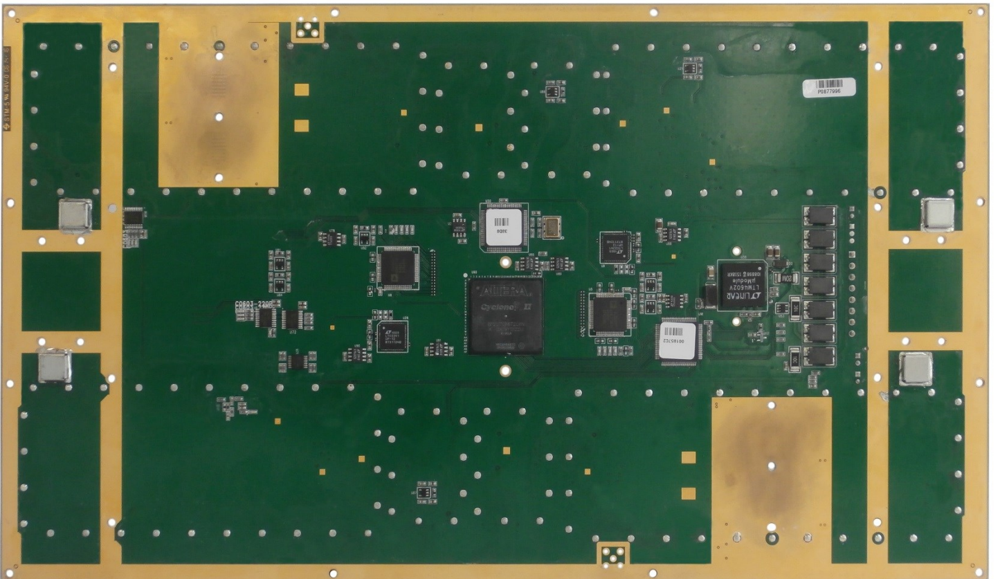
R010-2114-005 Non-Component Side
