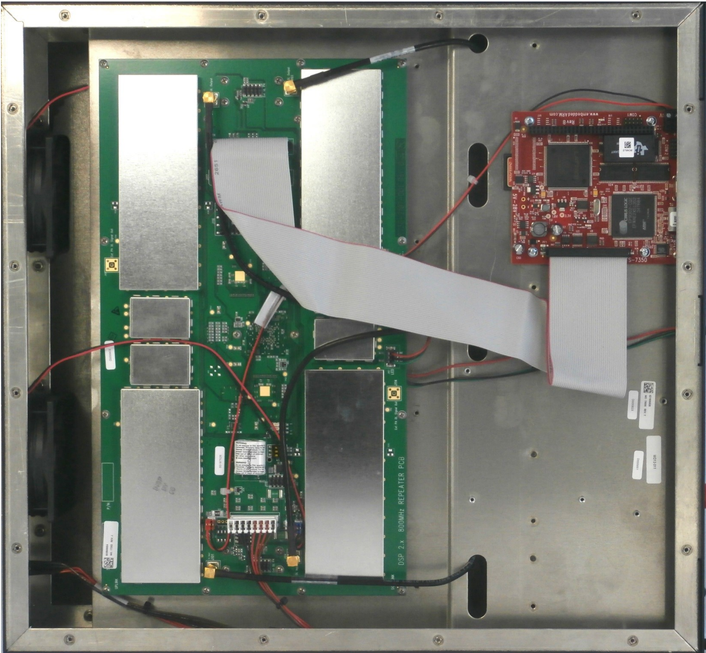
Chassis SBC Side Cover Off
