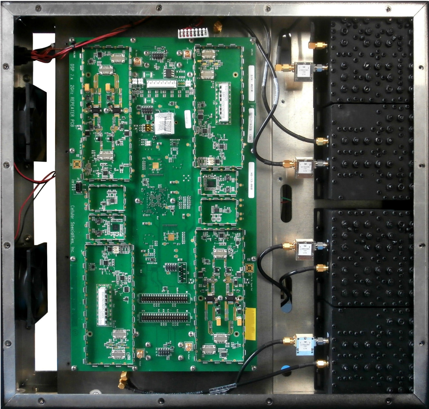
Chassis Diplexer Side Cover Off
