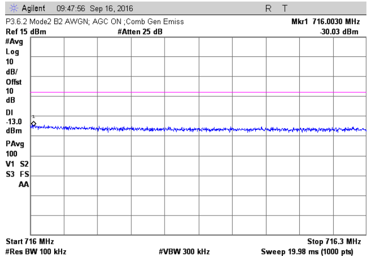
AWGN; 708.5 +713.5 MHz Injected Signals; AGC on
