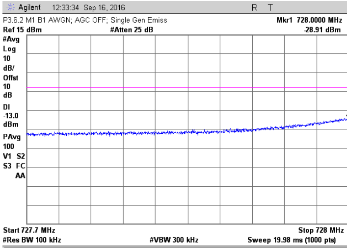
AWGN; 730.5 MHz Injected Signal; AGC off
