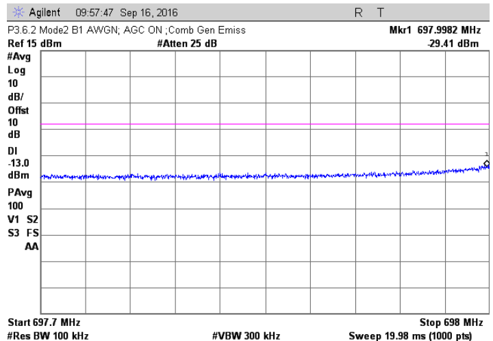
AWGN; 700.5 +705.5 MHz Injected Signals; AGC on
