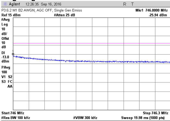
AWGN; 743.5 MHz Injected Signal; AGC off
