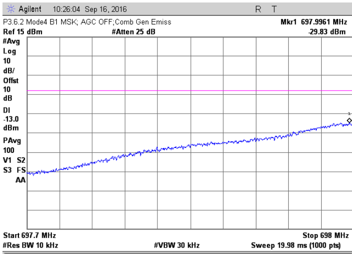
MSK; 698.2 +698.4 MHz Injected Signals; AGC off
