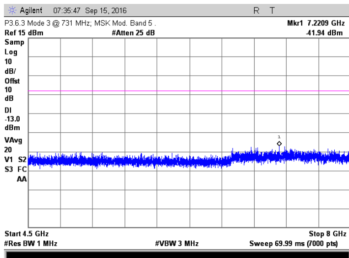
MSK; 731 MHz Injected Signal
