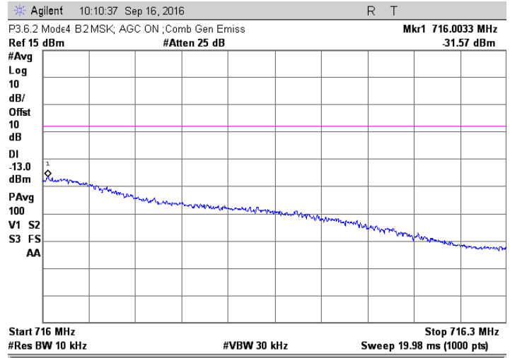
MSK; 715.6 +715.8 MHz MHz Injected Signals; AGC on
