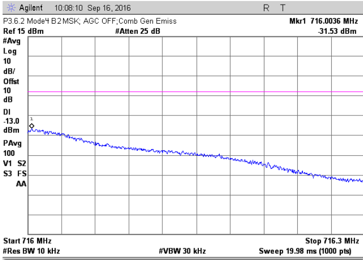
MSK; 715.6 +715.8 MHz Injected Signals; AGC off
