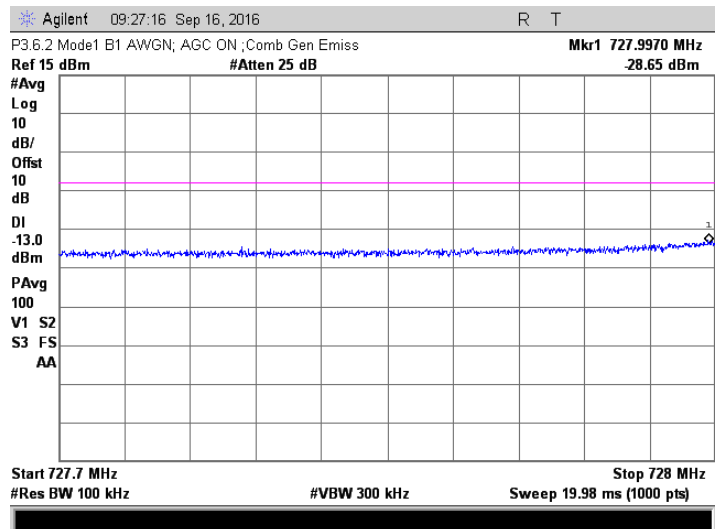
AWGN; 730.5 +735.5 MHz Injected Signals; AGC on
