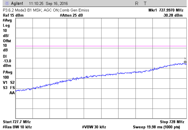
MSK; 728.2 +728.4 MHz Injected Signals; AGC on
