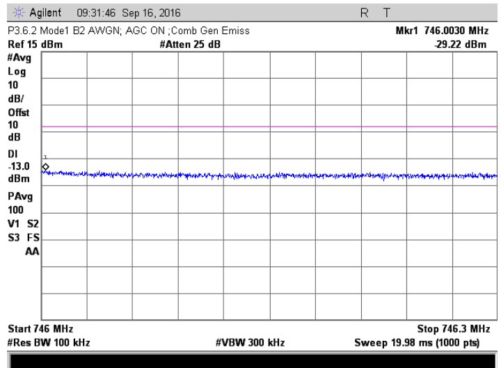
AWGN; 738.5 +743.5 MHz Injected Signals; AGC on
