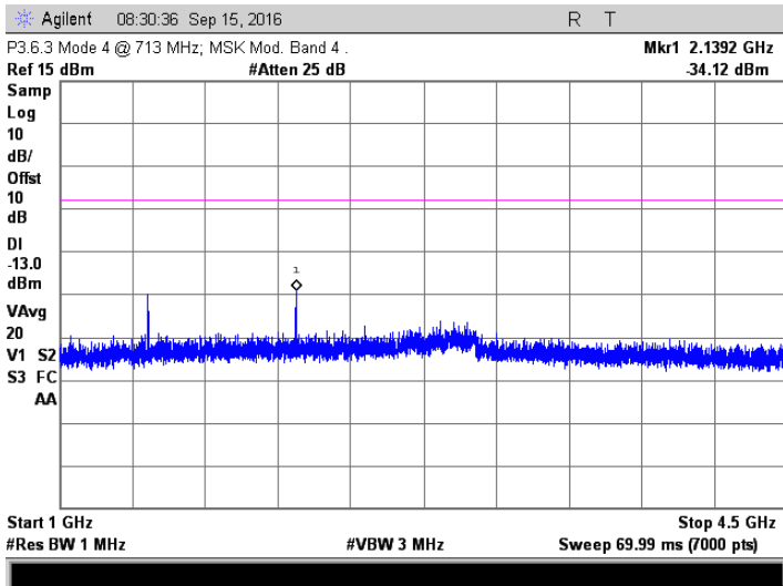
MSK; 713 MHz Injected Signal
