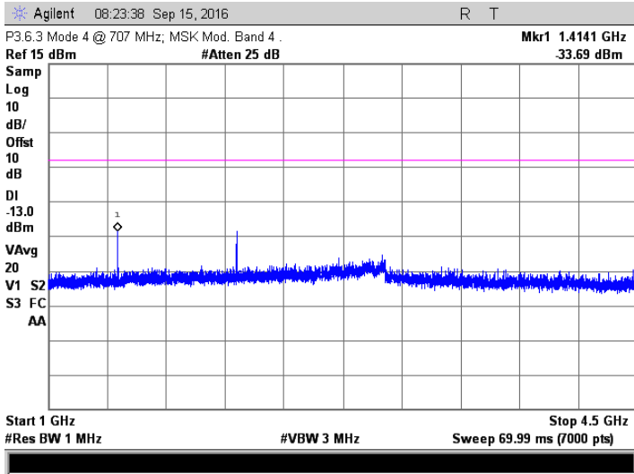
MSK; 707 MHz Injected Signal
