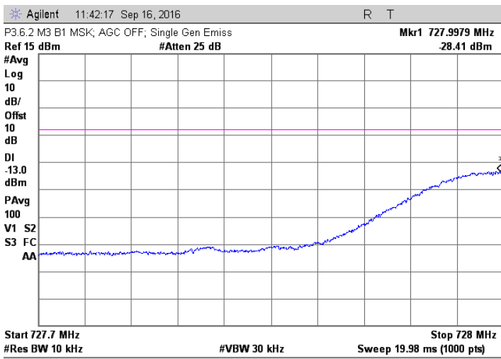
MSK; 728.2 MHz Injected Signal; AGC off
