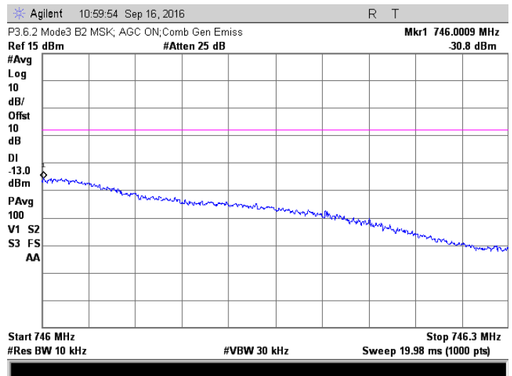
MSK; 745.6 +745.8 MHz Injected Signals; AGC on
