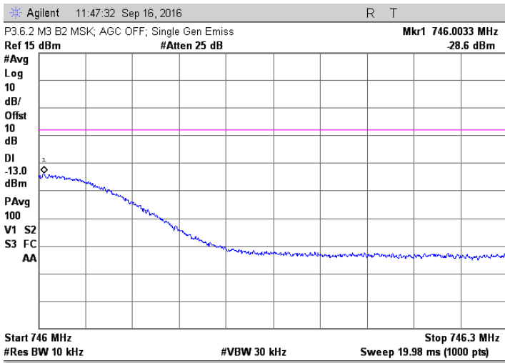
MSK; 745.8 MHz Injected Signal; AGC off
