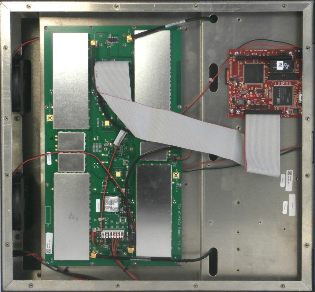
CHASSIE TOP
