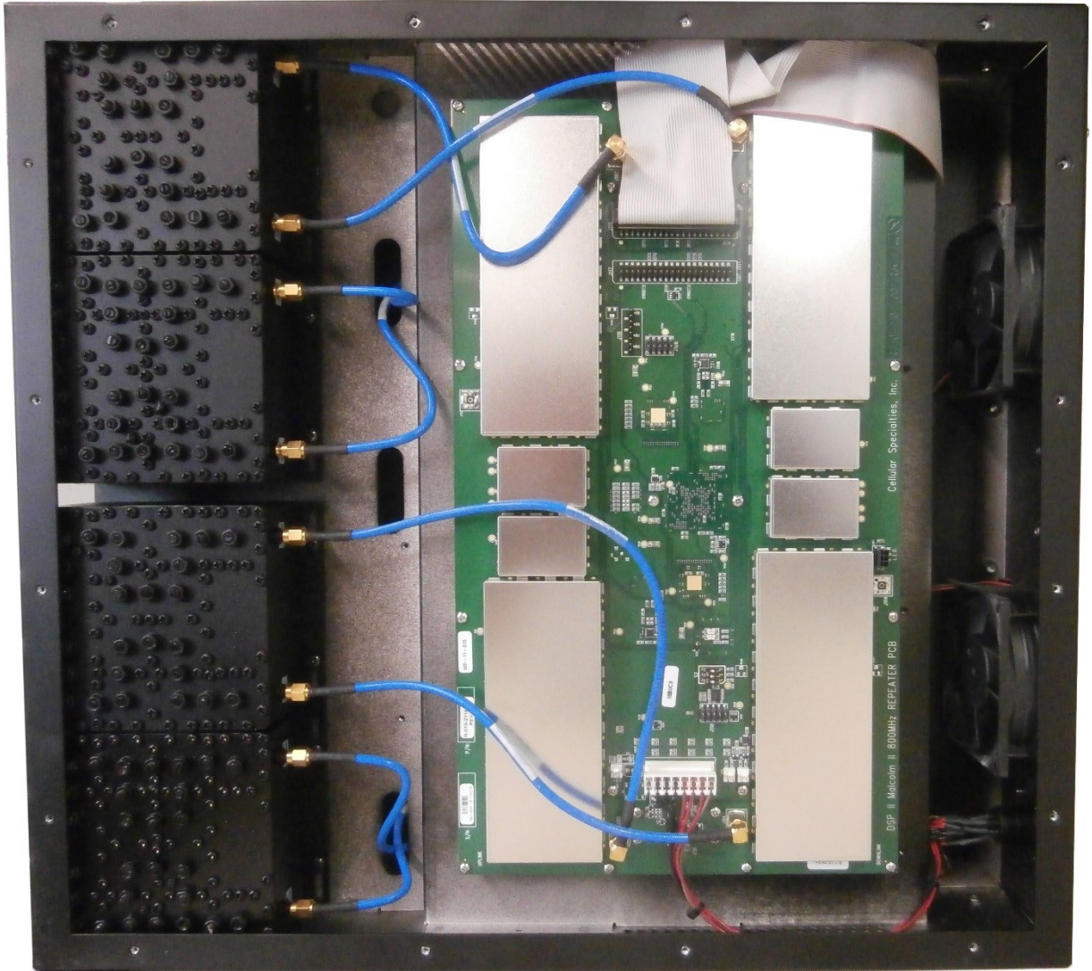
CHASSIE BOTTOM
