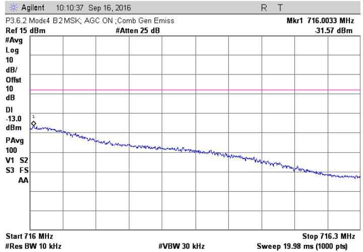
MSK; 715.6 +715.8 MHz Injected Signals; AGC on
