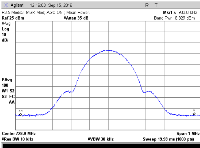
728.9 MHz MSK; AGC On
