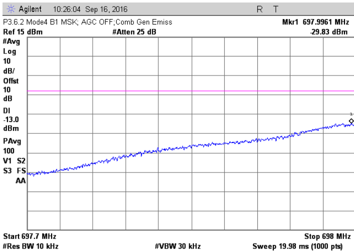
MSK; 698.2 +698.4 MHz Injected Signals; AGC off
