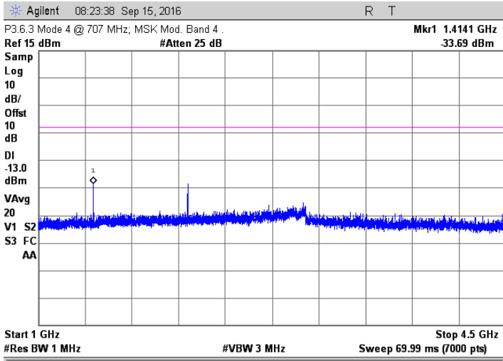
MSK; 707 MHz Injected Signal
