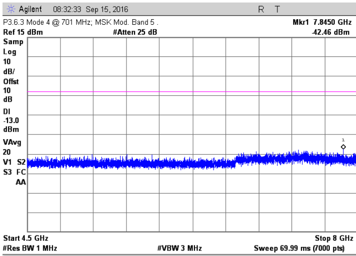
MSK; 701 MHz Injected Signal
