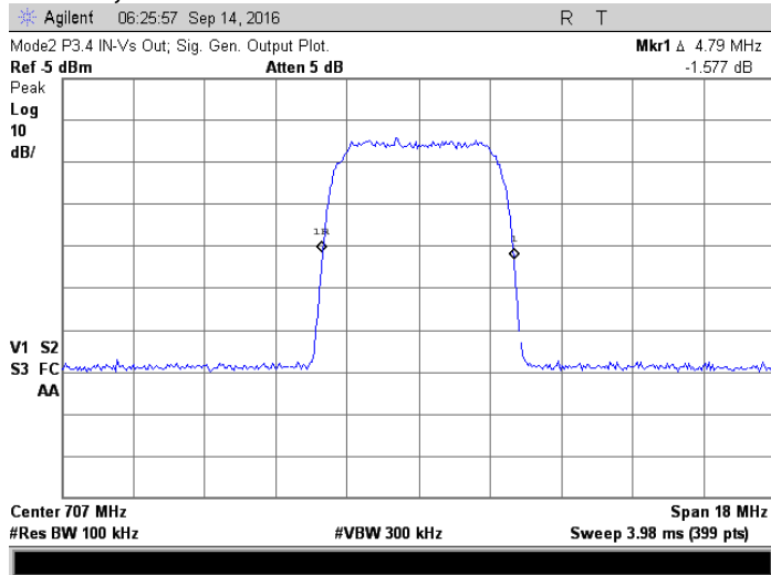
Generator output; 707 MHz, AWGN
