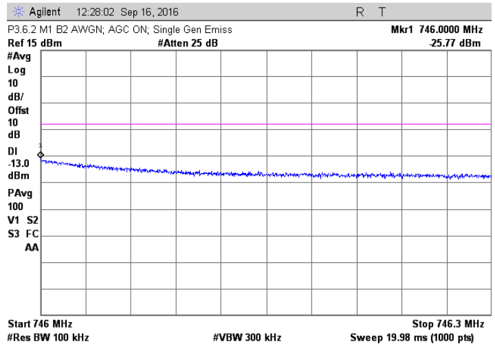
AWGN; 743.5 MHz Injected Signal; AGC on
