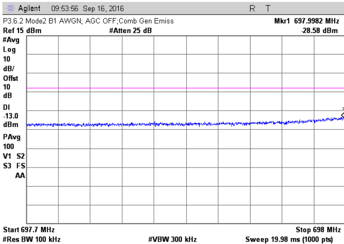
AWGN; 700.5 +705.5 MHz Injected Signals; AGC off
