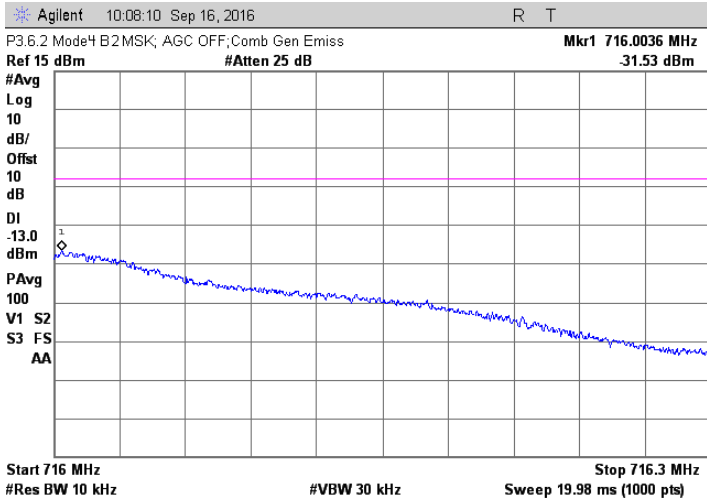
MSK; 715.6 +715.8 MHz Injected Signals; AGC off
