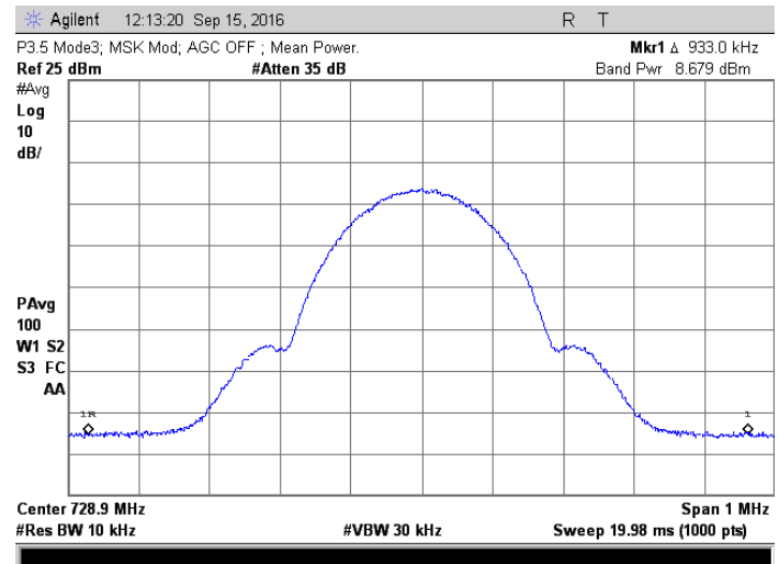
728.9 MHz; MSK; AGC off
