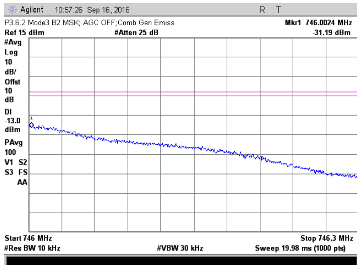
MSK; 745.6 +745.8 MHz Injected Signals; AGC off
