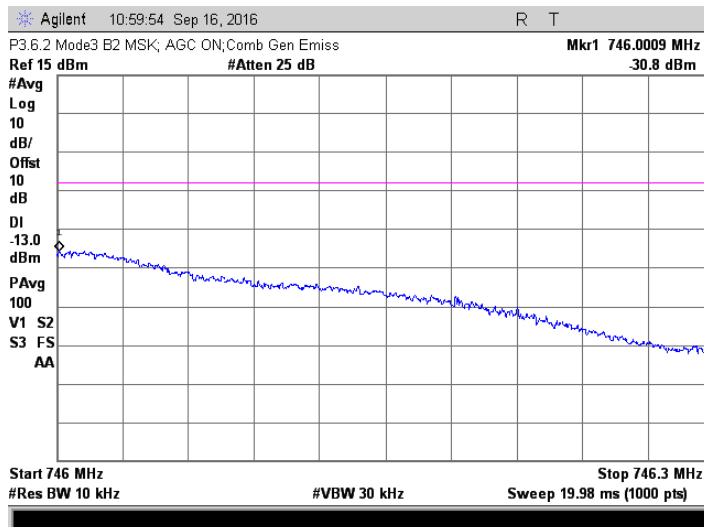
MSK; 745.6 +745.8 MHz MHz Injected Signals; AGC on
