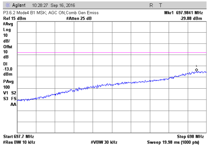
MSK; 698.2 +698.4 MHz Injected Signals; AGC on
