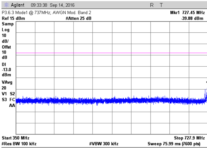
AWGN; 737 MHz Injected Signal
