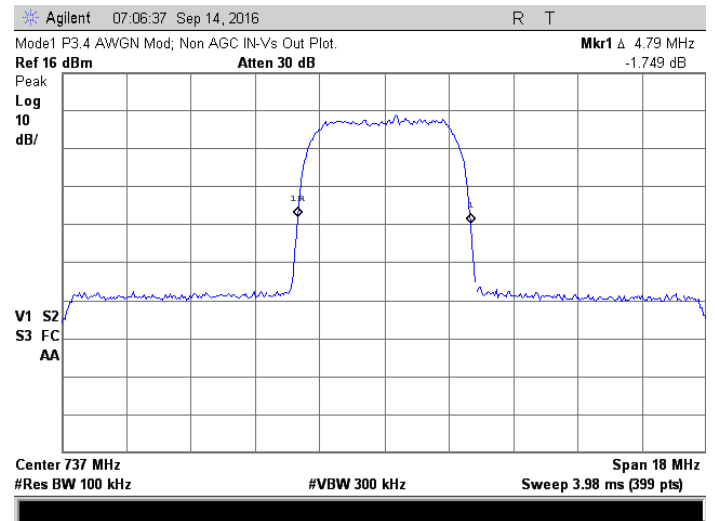
Amp output, no AGC; 737 MHz, AWGN
