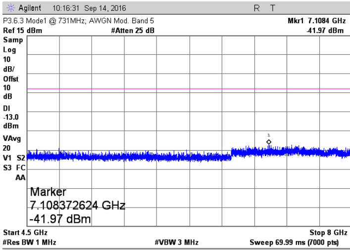
AWGN; 731 MHz Injected Signal
