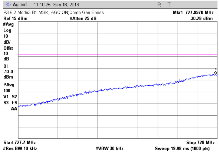
MSK; 728.2 +728.4 MHz MHz Injected Signals; AGC on
