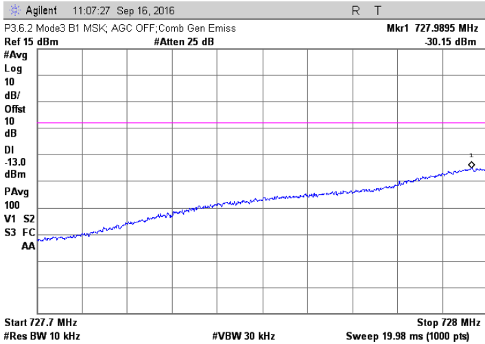
MSK; 728.2 +728.4 MHz Injected Signals; AGC off
