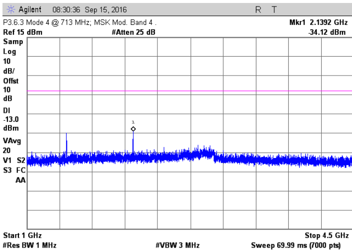
MSK; 713 MHz Injected Signal
