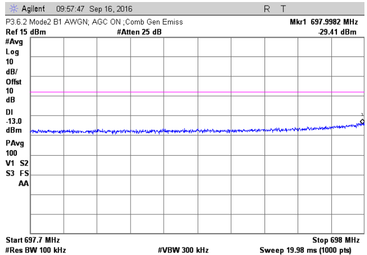
AWGN; 700.5 +705.5 MHz MHz Injected Signals; AGC on
