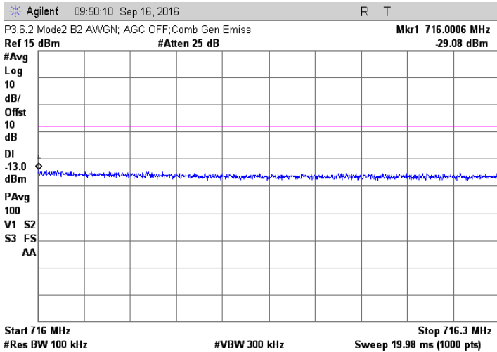
AWGN; 708.5 +713.5 MHz Injected Signals; AGC off
