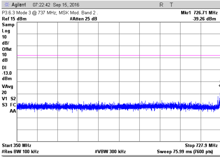
MSK; 737 MHz Injected Signal
