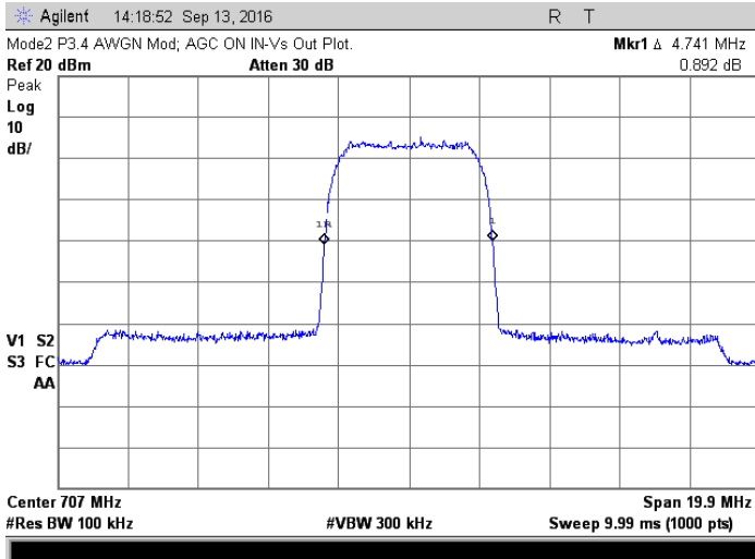
Amp output with AGC; 707 MHz, AWGN
