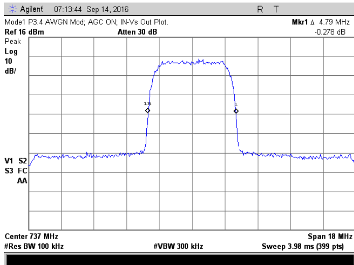
Amp output with AGC; 737 MHz, AWGN
