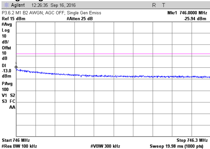
AWGN; 743.5 MHz Injected Signal; AGC off
