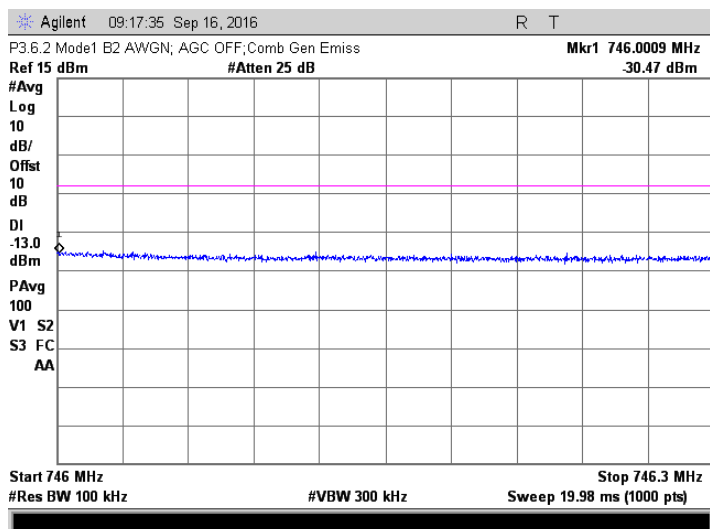
AWGN; 738.5 +743.5 MHz Injected Signals; AGC off
