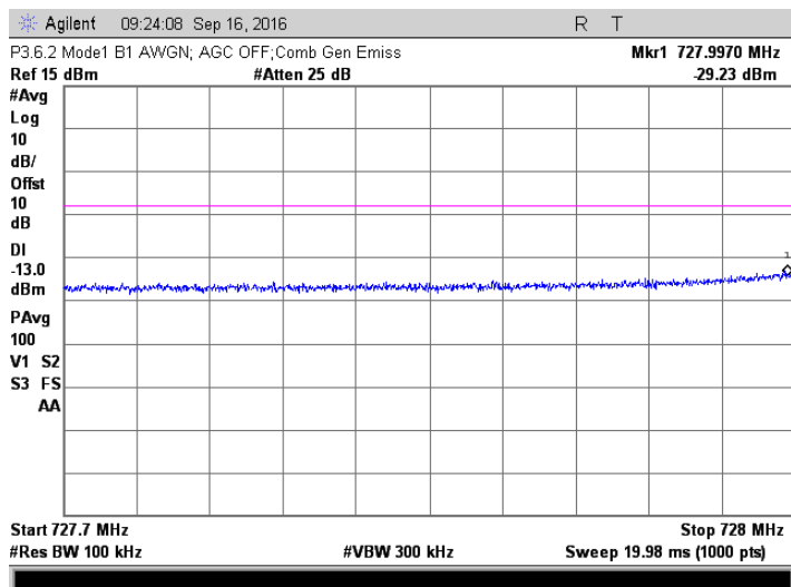
AWGN; 730.5 +735.5 MHz Injected Signals; AGC off
