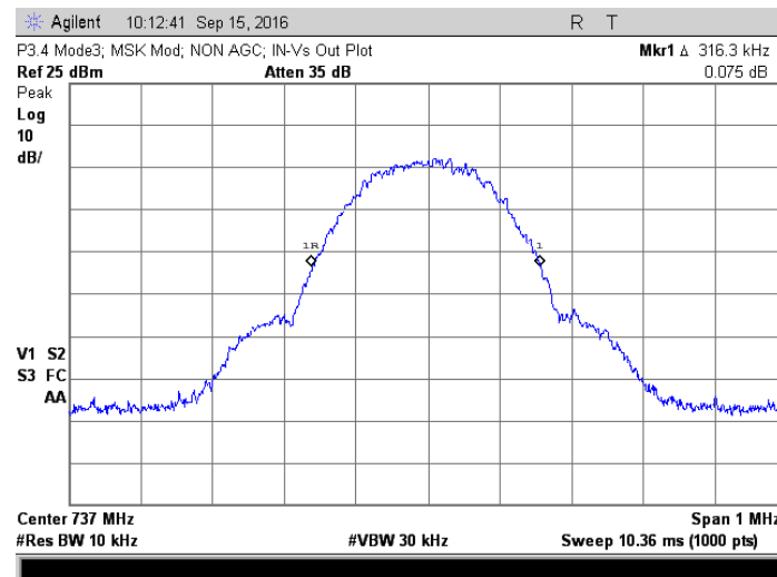
Amp output, no AGC; 737 MHz, MSK
