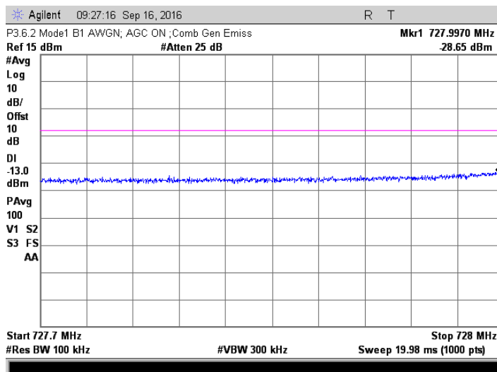
AWGN; 730.5 +735.5 MHz Injected Signals; AGC on
