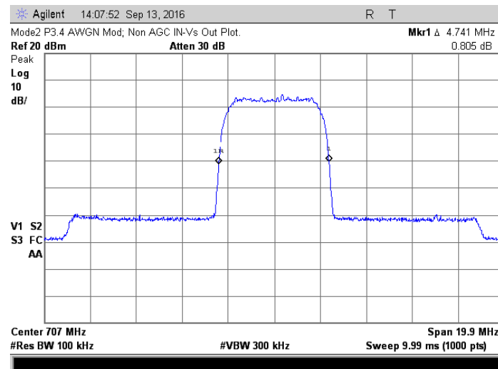
Amp output, no AGC; 707 MHz, AWGN
