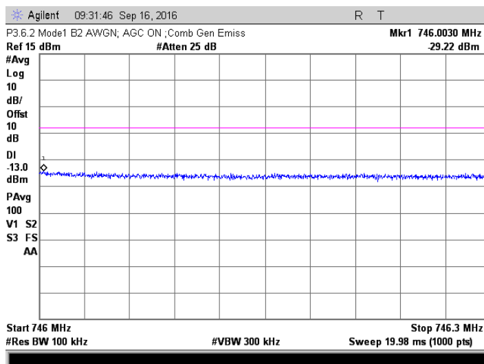
AWGN; 738.5 +743.5 MHz Injected Signals; AGC on
