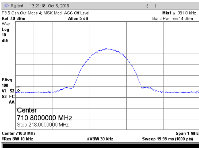
710.8 MHz MSK; Generator Out
