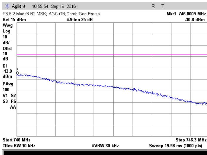
MSK; 745.6 +745.8 MHz Injected Signals; AGC on
