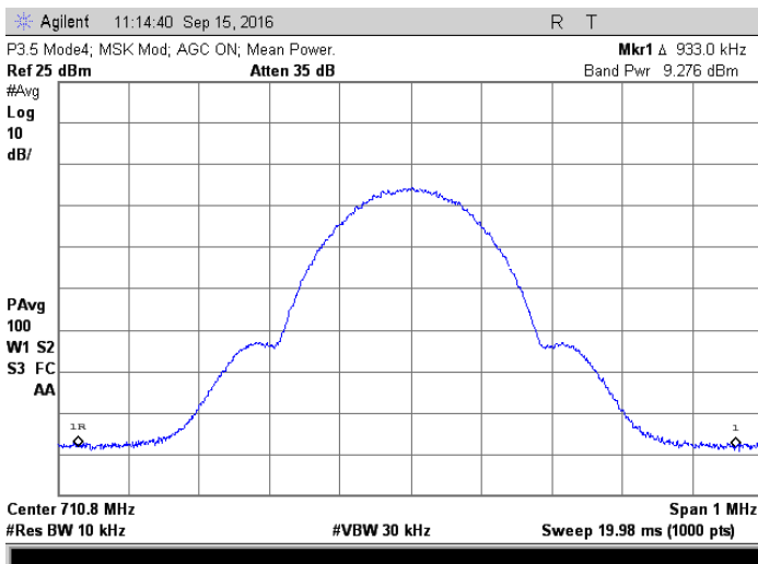
710.8 MHz MSK; AGC On
