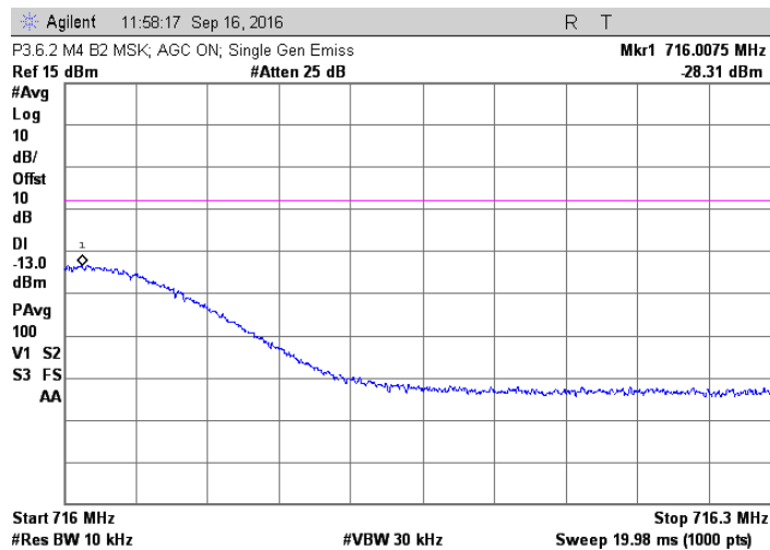
MSK; 715.8 MHz Injected Signal; AGC on
