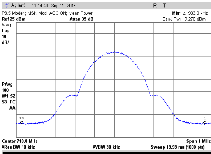
710.8 MHz MSK; AGC On
