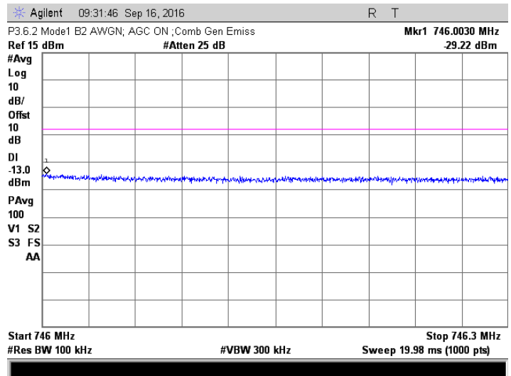
AWGN; 738.5 +743.5 MHz MHz Injected Signals; AGC on
