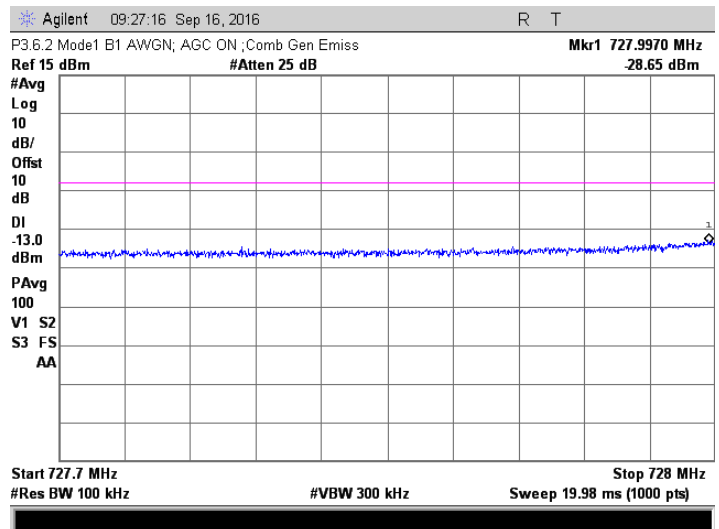
AWGN; 730.5 +735.5 MHz MHz Injected Signals; AGC on
