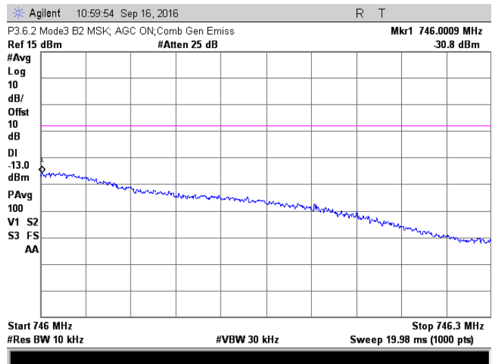
MSK; 745.6 +745.8 MHz MHz Injected Signals; AGC on
