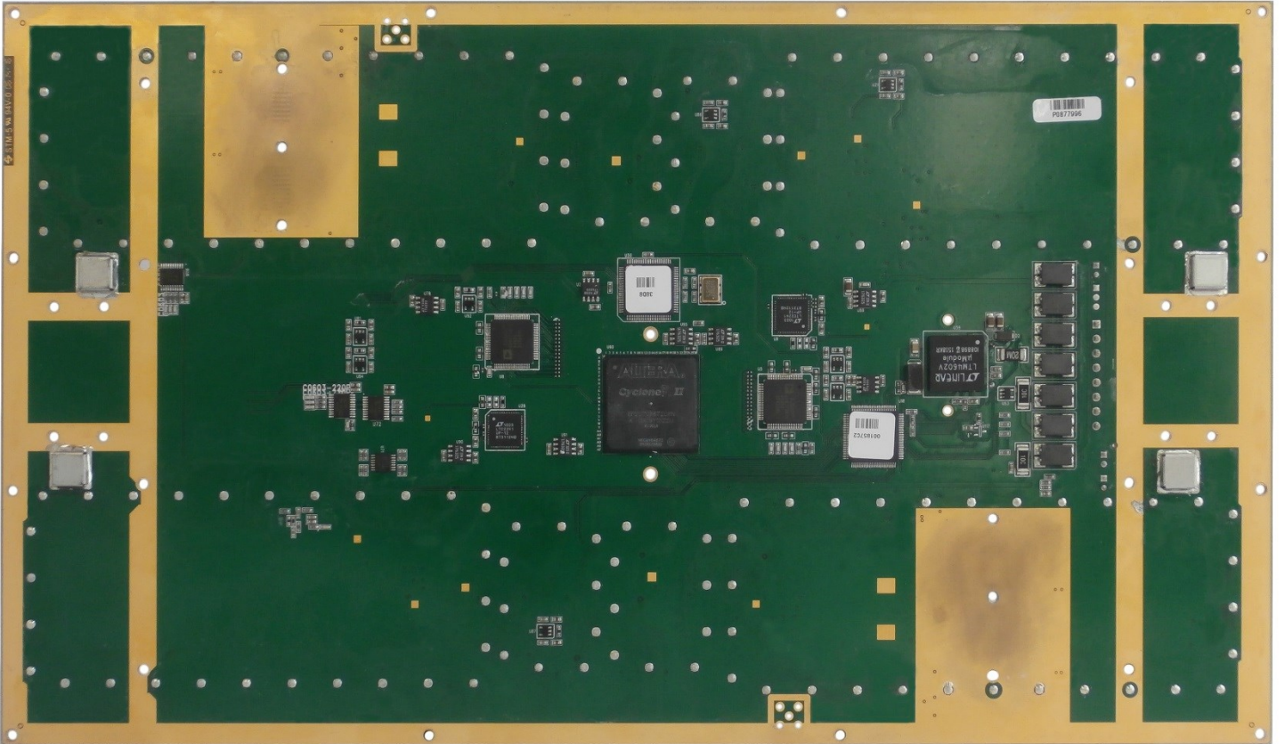
AWS PCB Non-Component Side
