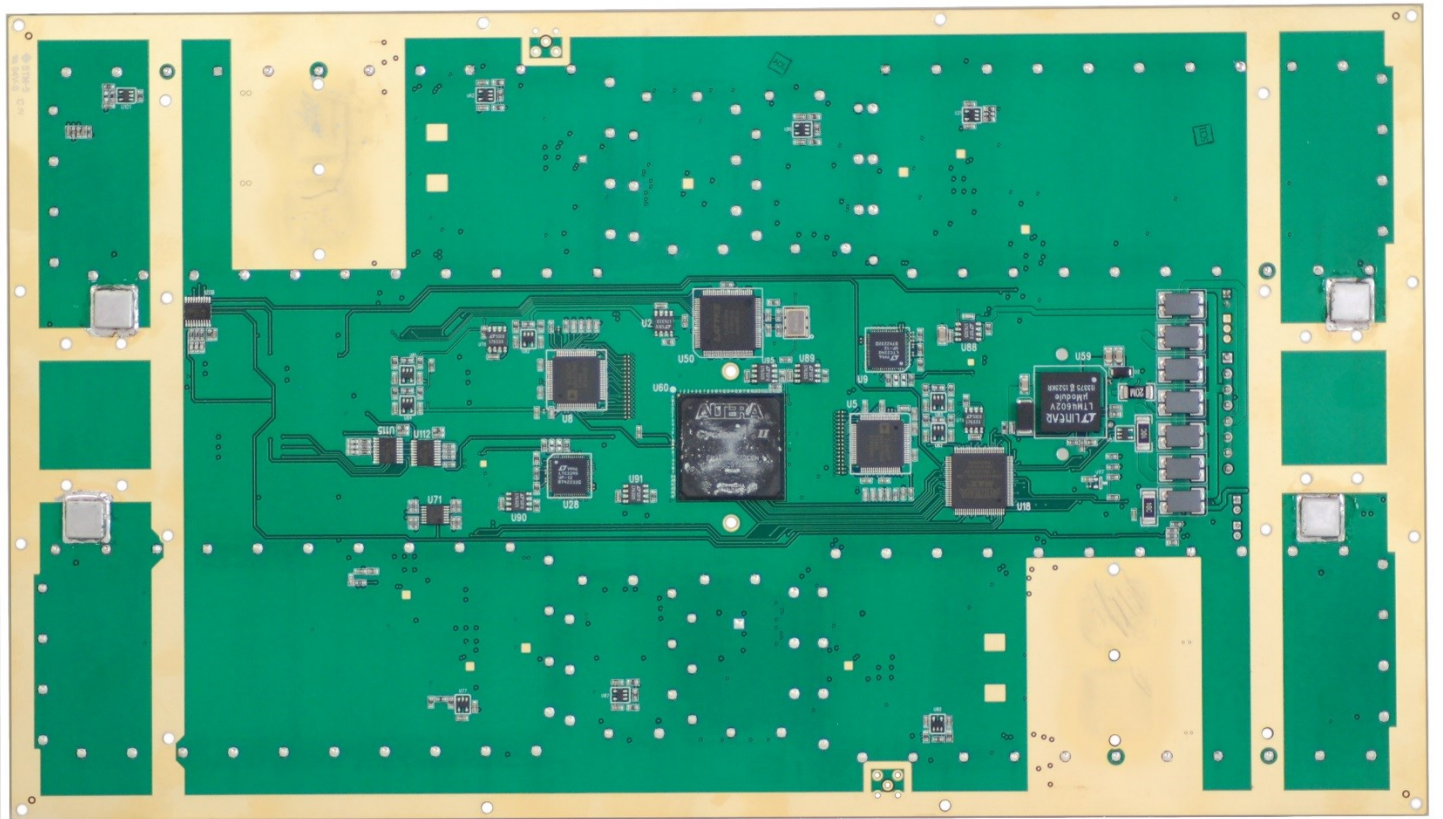
L7 PCB Non-Component Side
