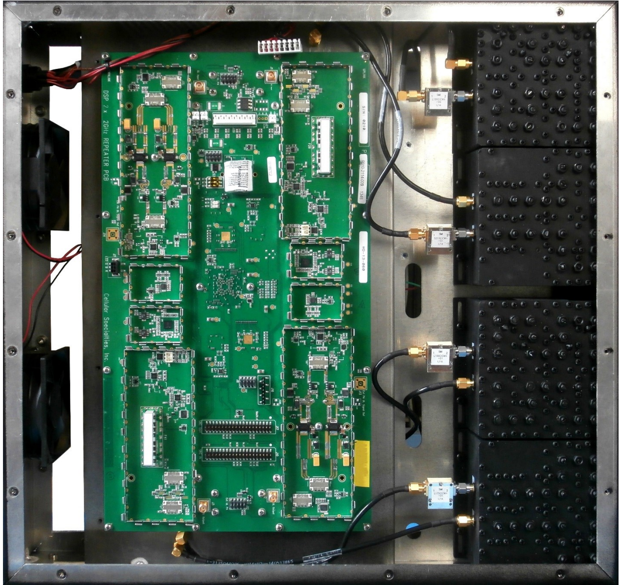
Chassis Bottom View
