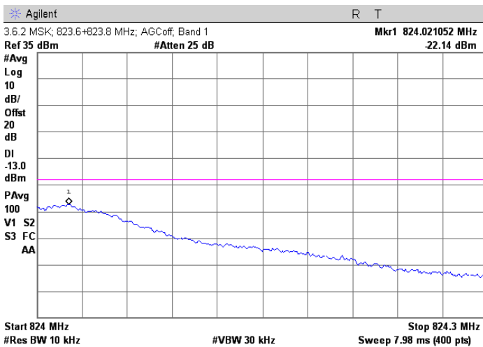
MSK; 823.6 + 823.8 MHz Injected Signals; AGC off
