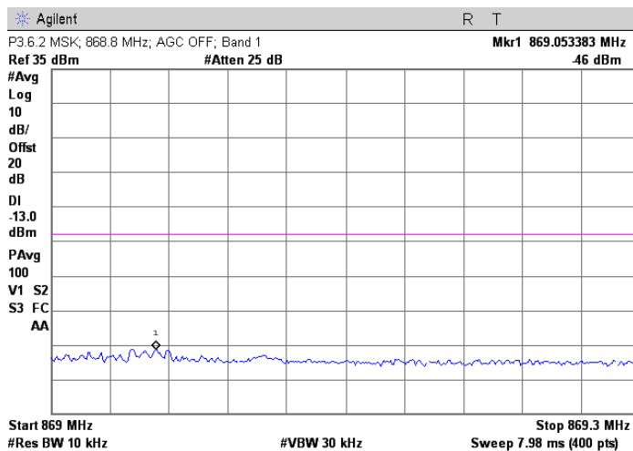
MSK; 868.8 MHz Injected Signal; AGC off
