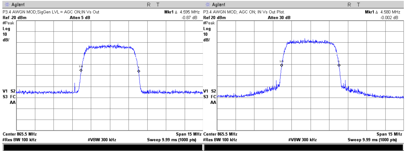
Generator output for AGC On ; 865.5 MHz, AWGN
