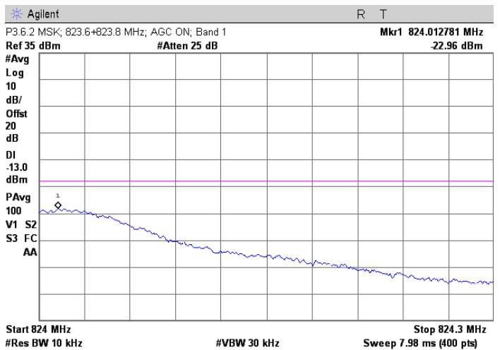
MSK; 823.6 + 823.8 MHz Injected Signals; AGC on
