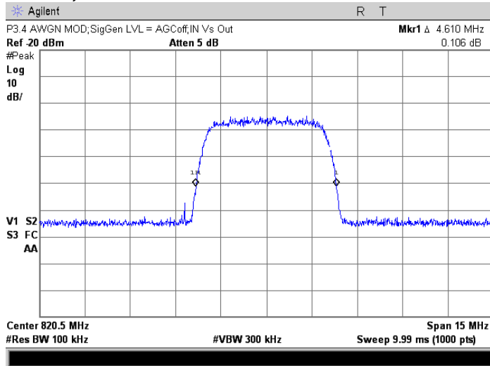
Generator output for AGC Off ; 820.5 MHz, AWGN
