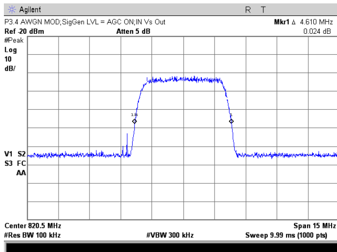
Generator output for AGC On ; 820.5 MHz, AWGN
