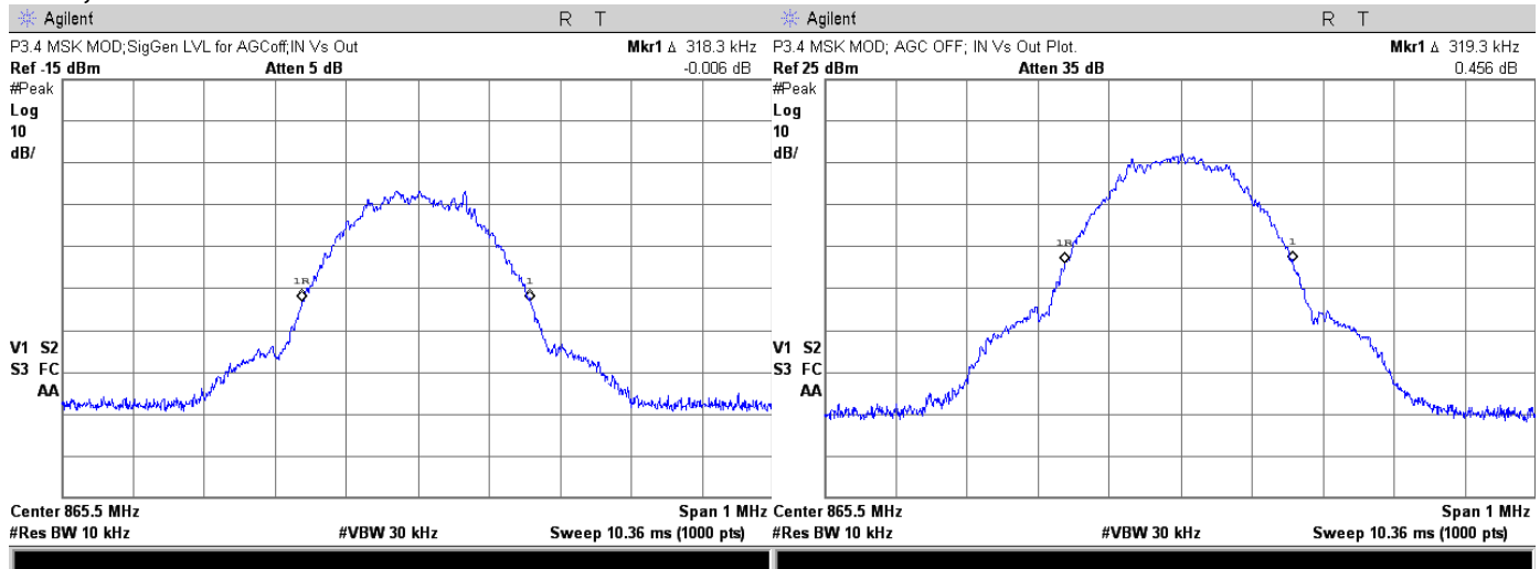
Generator output for AGC Off ; 865.5 MHz, MSK
