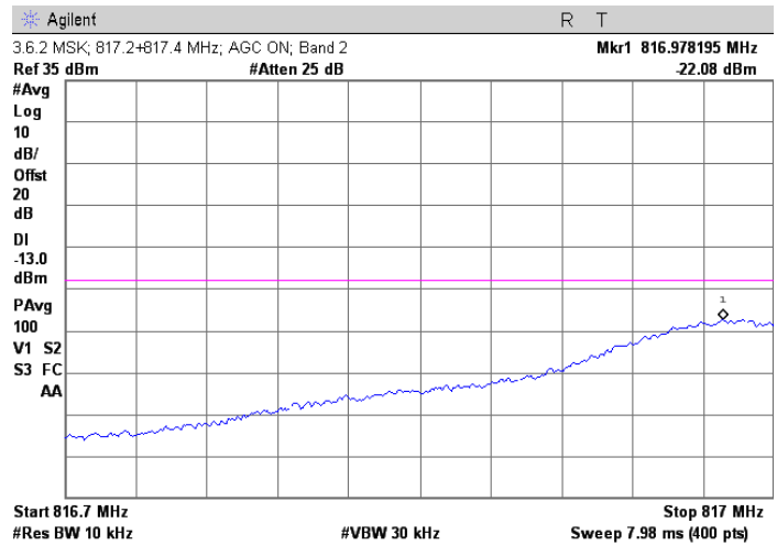
MSK; 817.2 + 817.4 MHz Injected Signals; AGC on
