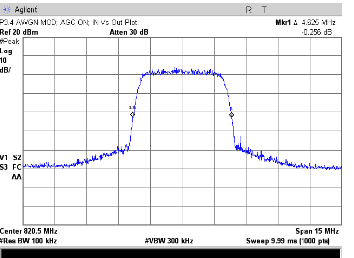
Amp output with AGC; 820.5 MHz, AWGN
