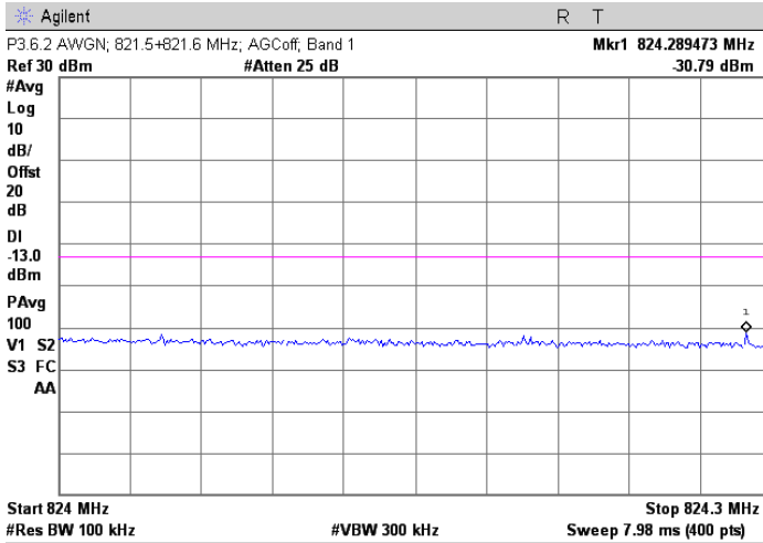
AWGN; 821.5 + 821.6 MHz Injected Signals; AGC off
