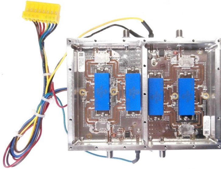
010-2043-001 COMP SIDE
