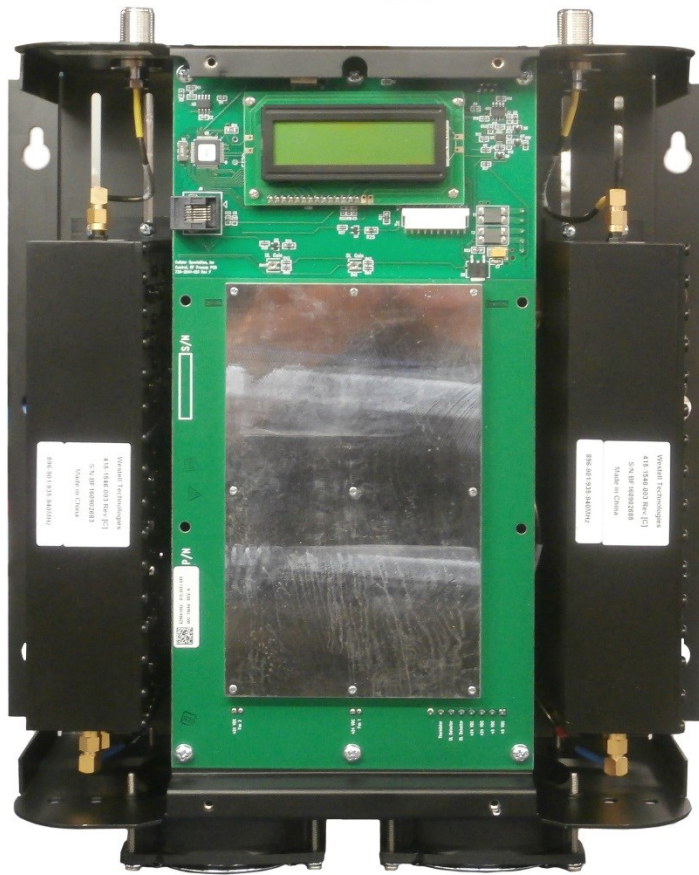
BDA610-P9 face on view cover off
