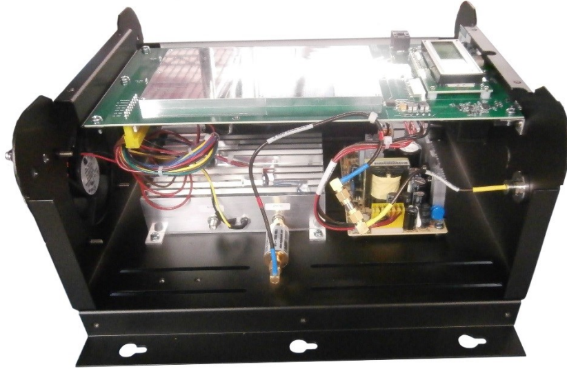
BDA610-P9 left side cover off
