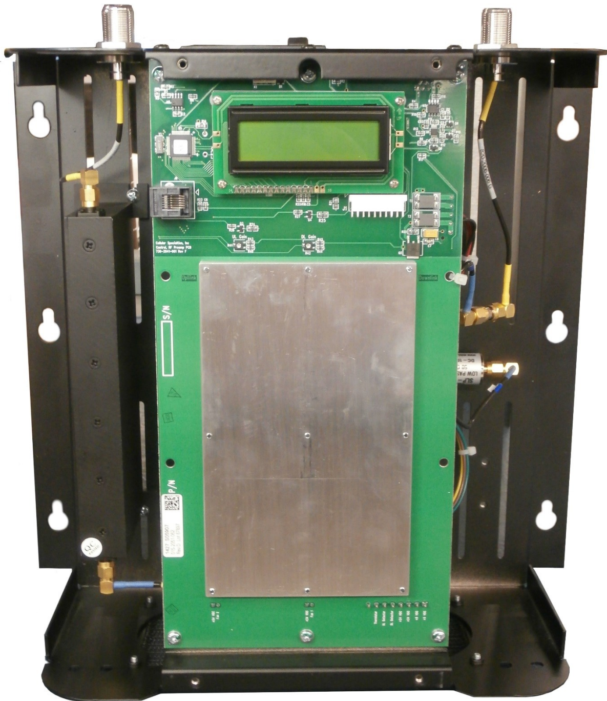
BDA510-P9 Face View Cover Off
