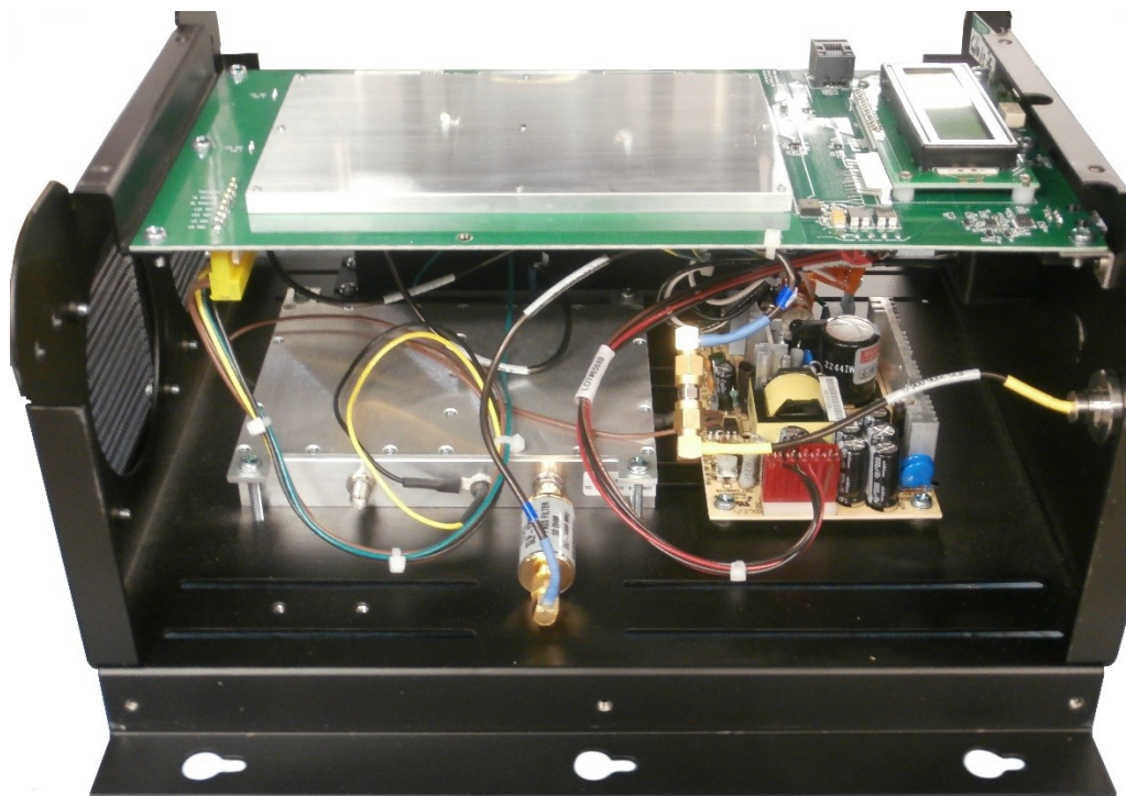
BDA510-P9 Left Side View Cover Off
