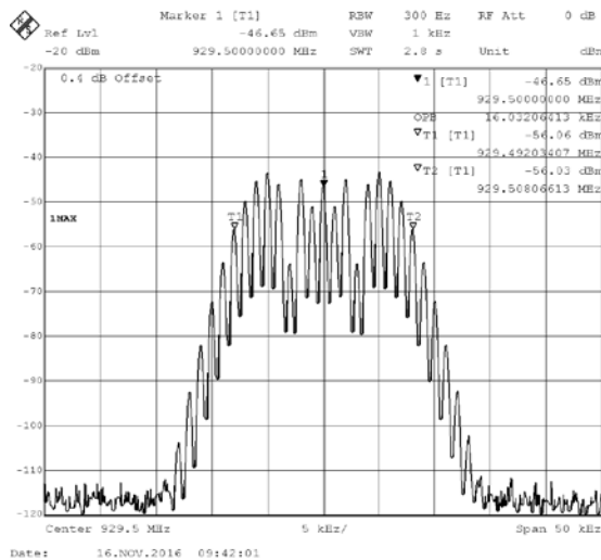
929.5 MHz 16K0F3E input (left) and output (right), level above AGC threshold
