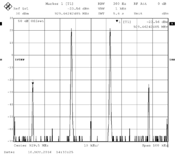
929-930MHz Out-of-band Emissions with 25kHz channel spacing, level below AGC (left) and above AGC (right)
