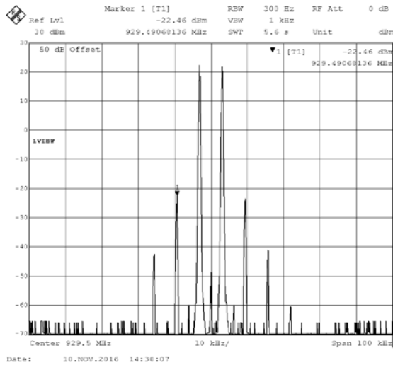
929-930MHz Out-of-band Emissions with 6.25kHz channel spacing, level below AGC (left) and above AGC (right)
