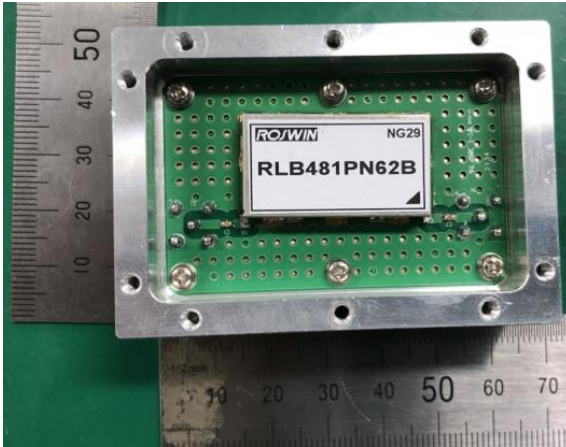
Top and Component Side
