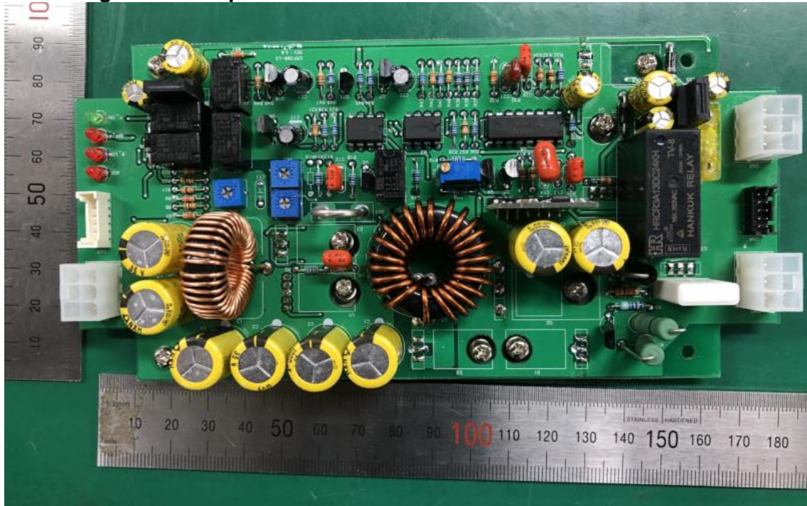
Photograph of Charger Board Bottom
