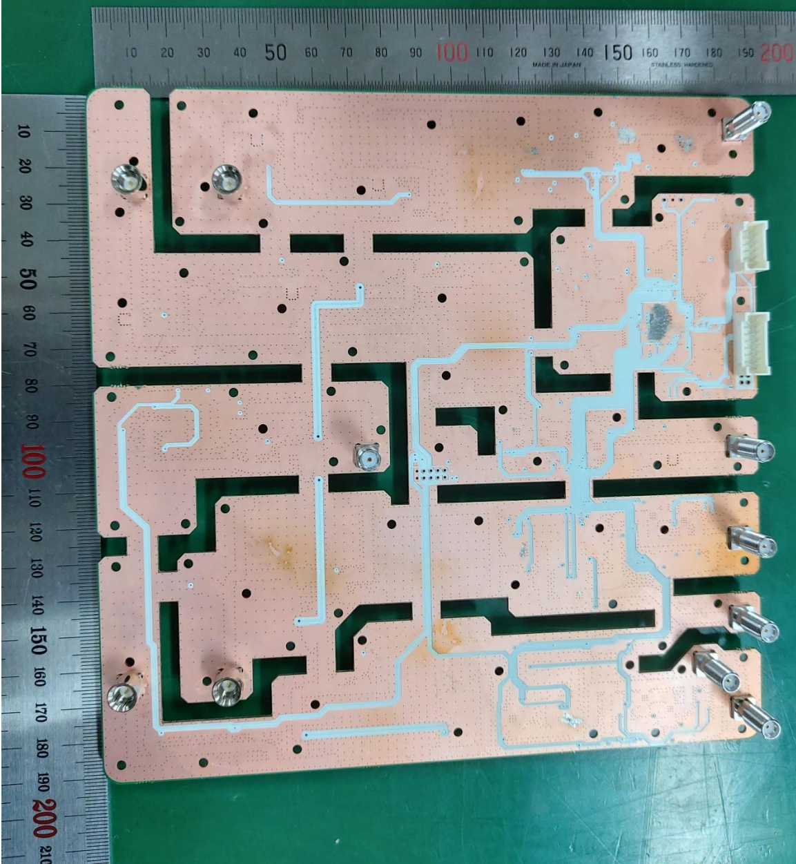
Photograph of UDCU Board: Foil Side
