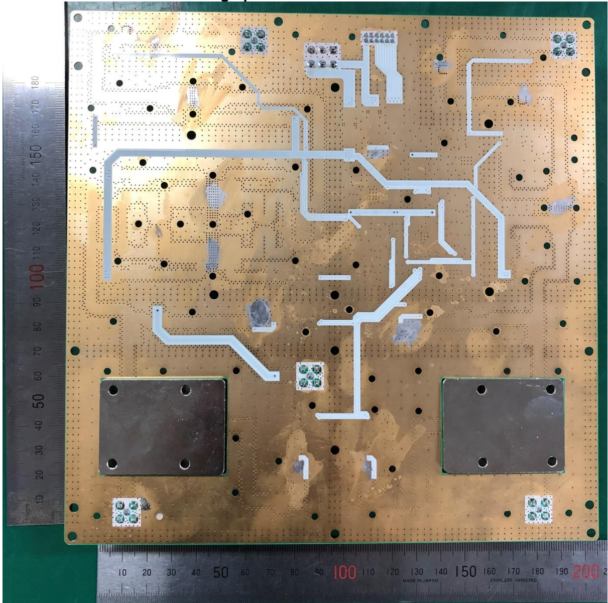
Photograph of HPA Board: Foil Side
