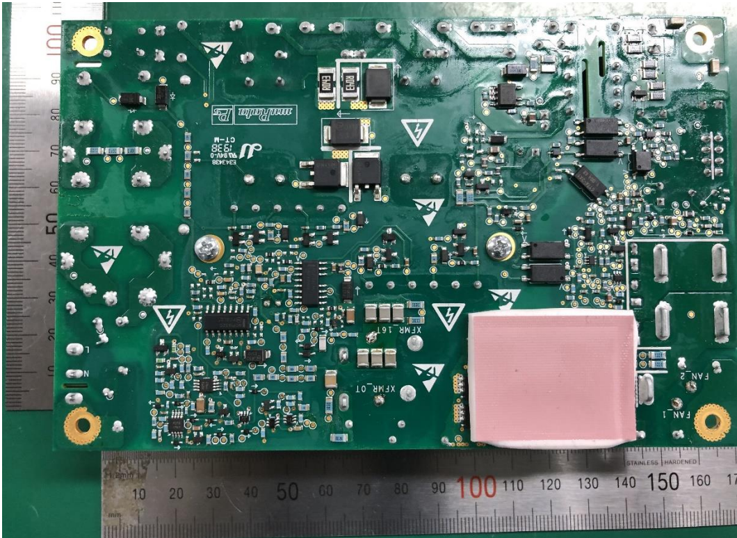
Photograph of PSU Bottom
