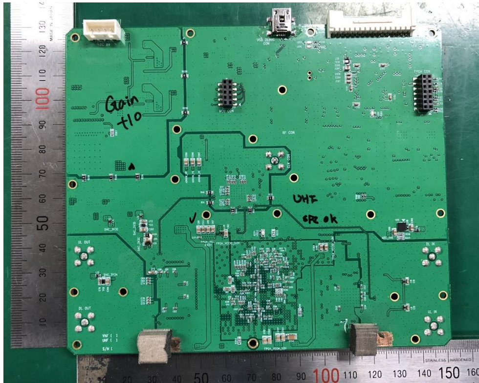
Photograph of DTU Board Bottom
