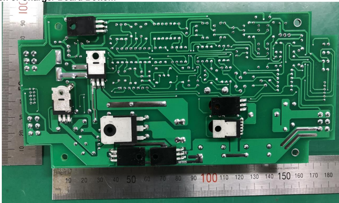
Photograph of Charger Board Bottom
