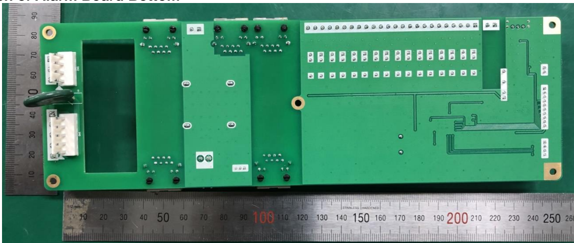
Photograph of Alarm Board Bottom
