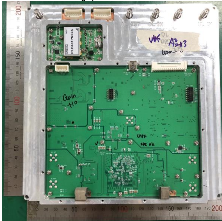
Detector Board Top
