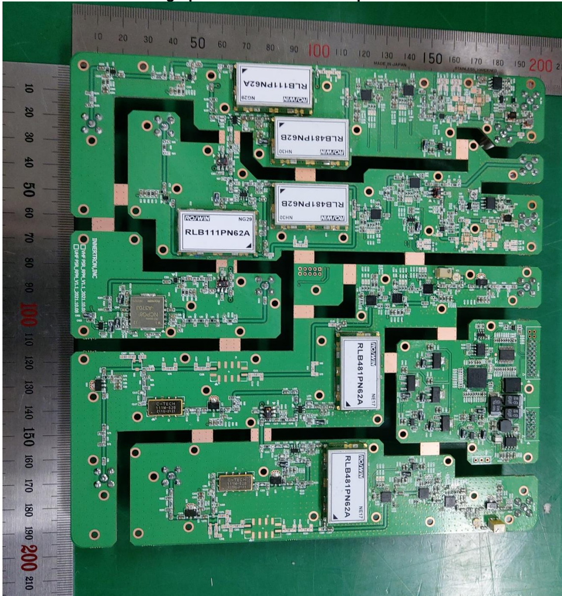
Photograph of UDCU Board: Component Side
