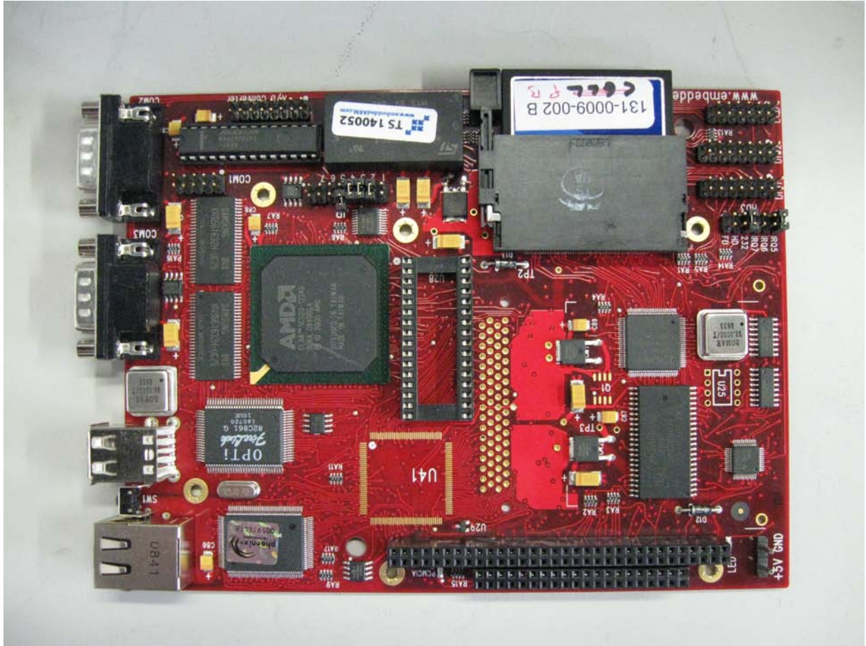
SBC Board - Front
