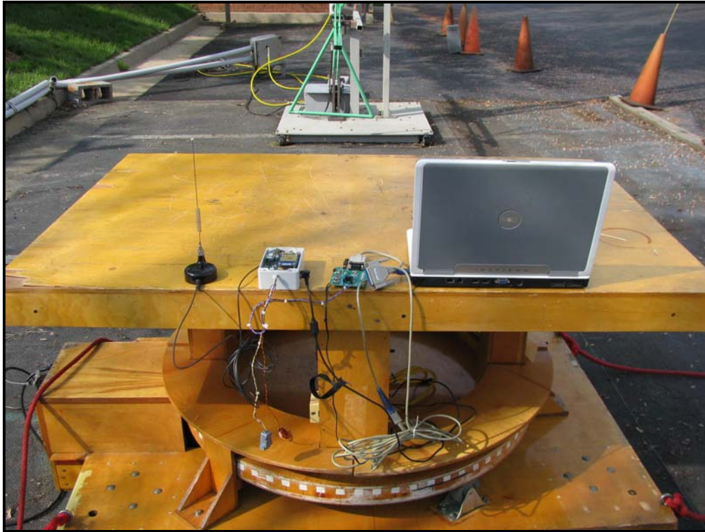
Photograph 3: Radiated Testing – Back View
