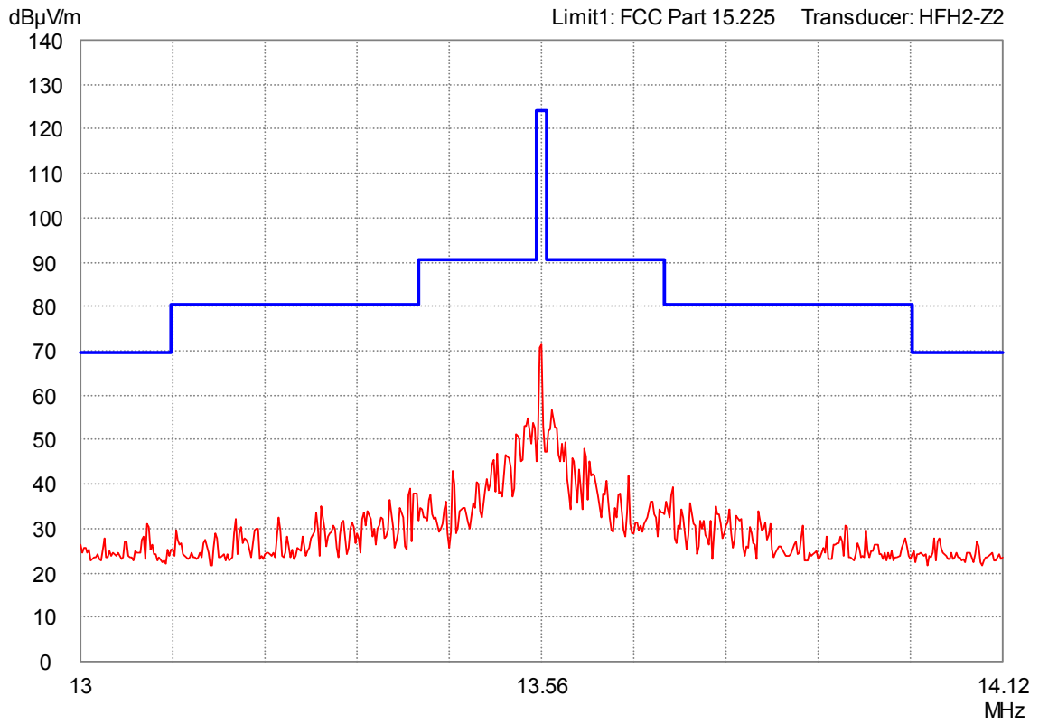
Figure 2: RBW = 1 kHz
