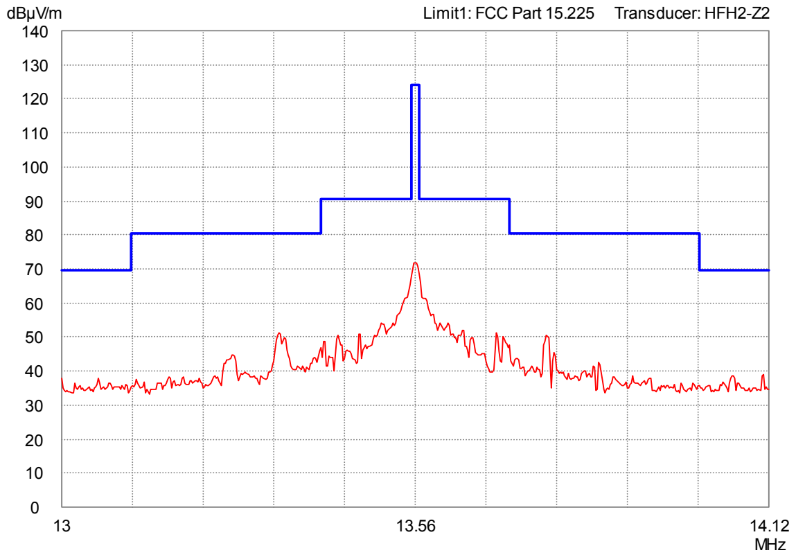
Figure 1: RBW = 10 kHz
