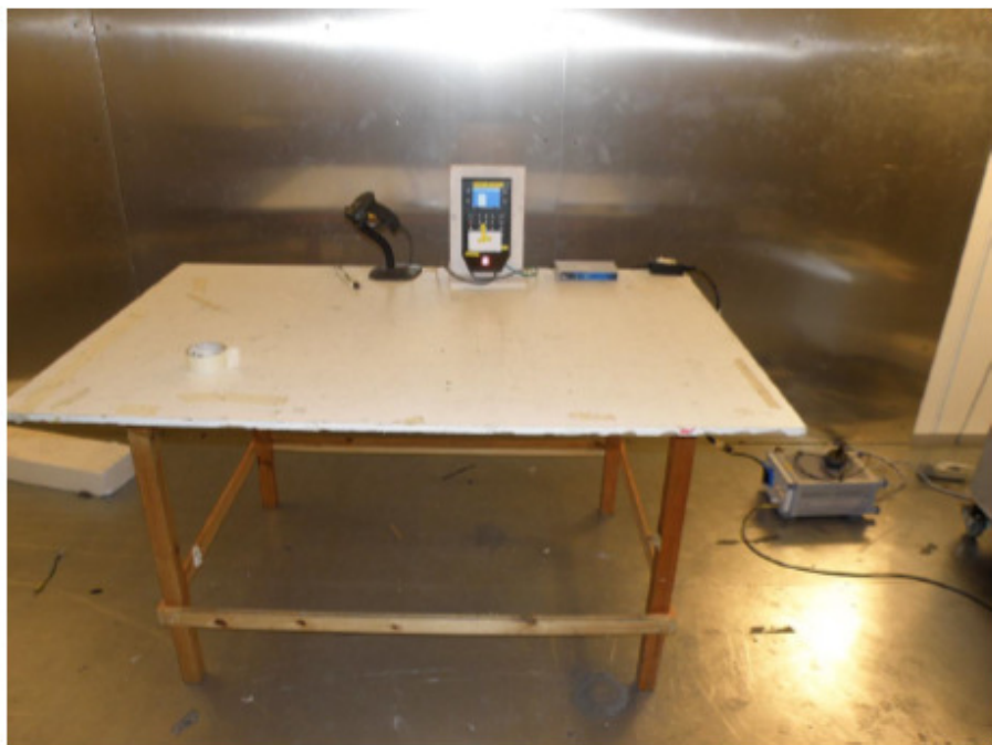
Photograph 4, AC mains conducted emissions test, configuration 2
