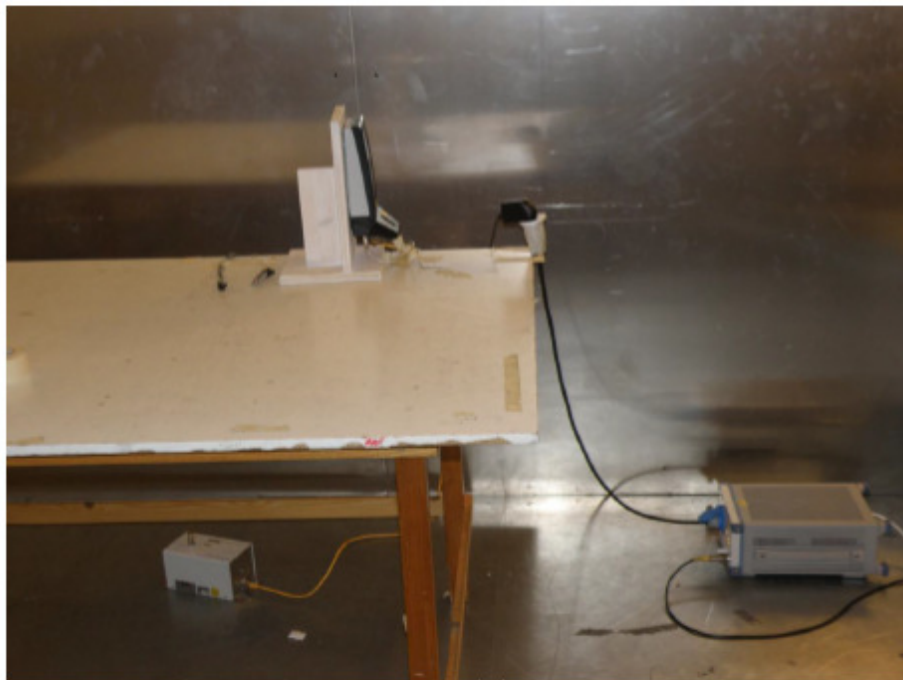
Photograph 2, AC mains conducted emissions test, configuration 1
