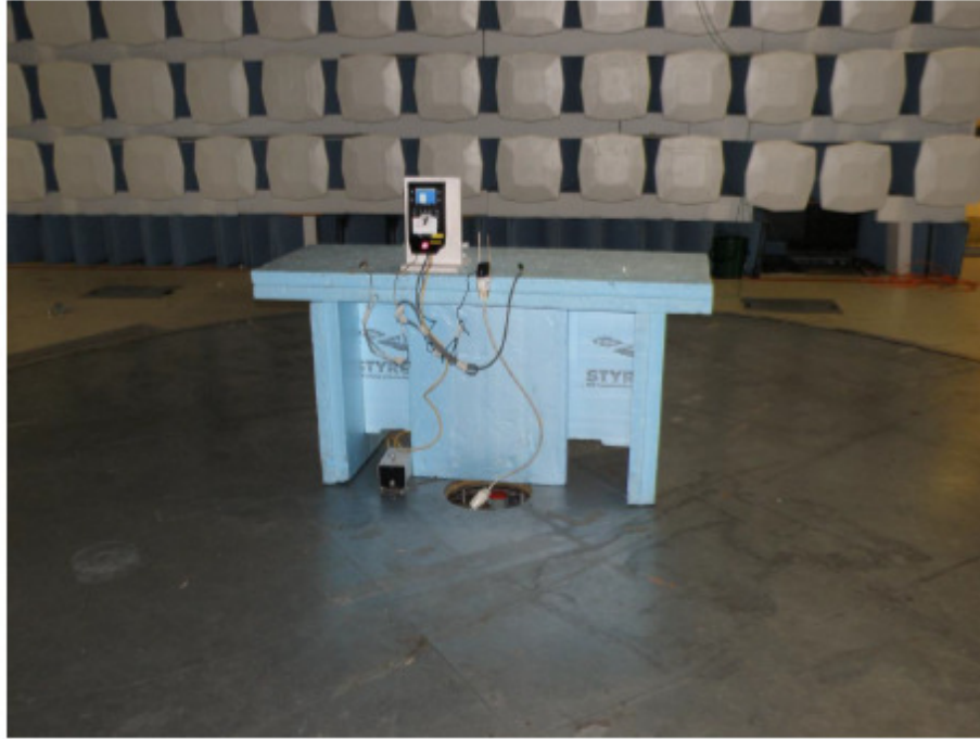
Photograph 1, Radiated emissions test, configuration 1
