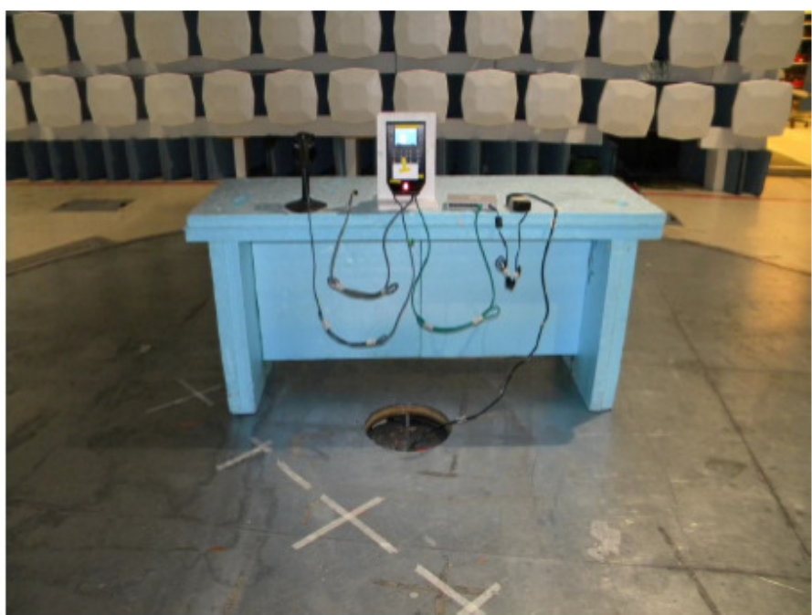
Photograph 3, Radiated emissions test, configuration 2
