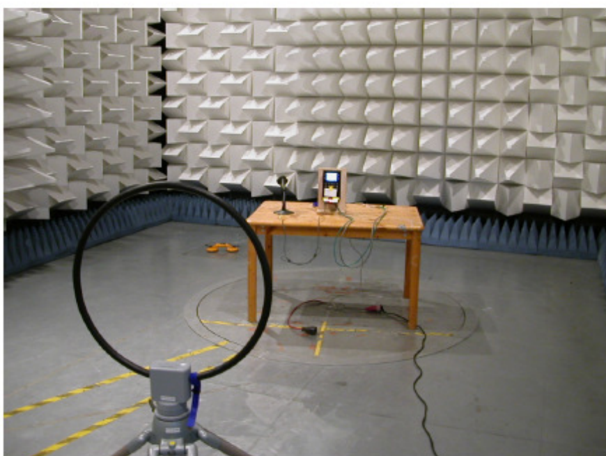
Figure 2 EUT / test set up - spurious radiated emissions
