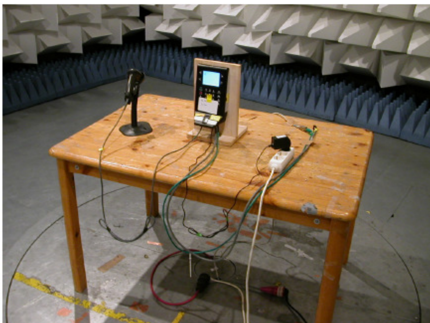
Figure 1 EUT / test set up - spurious radiated emissions
