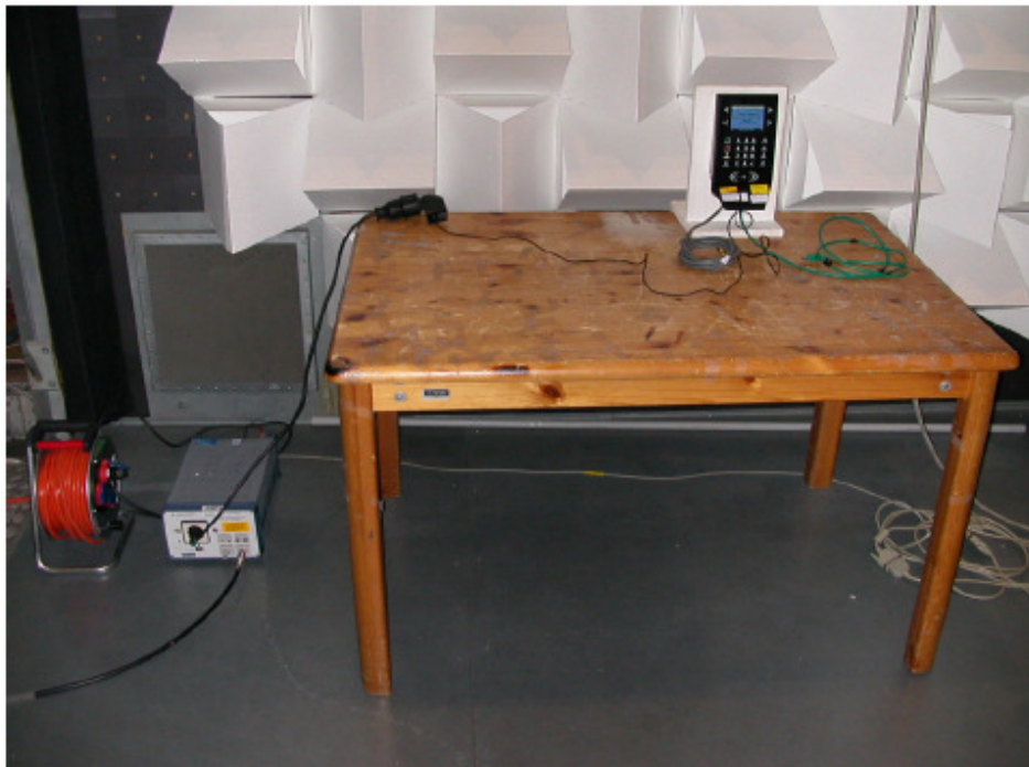
Figure 3 EUT / test set up - spurious conducted emissions
