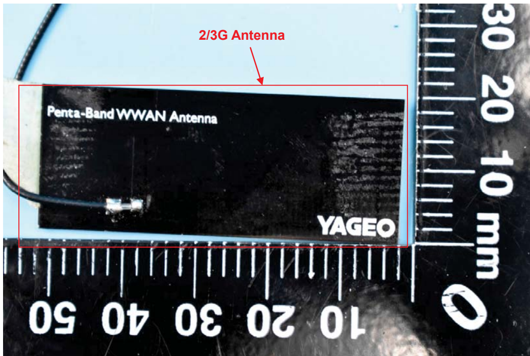
2. Antenna view
