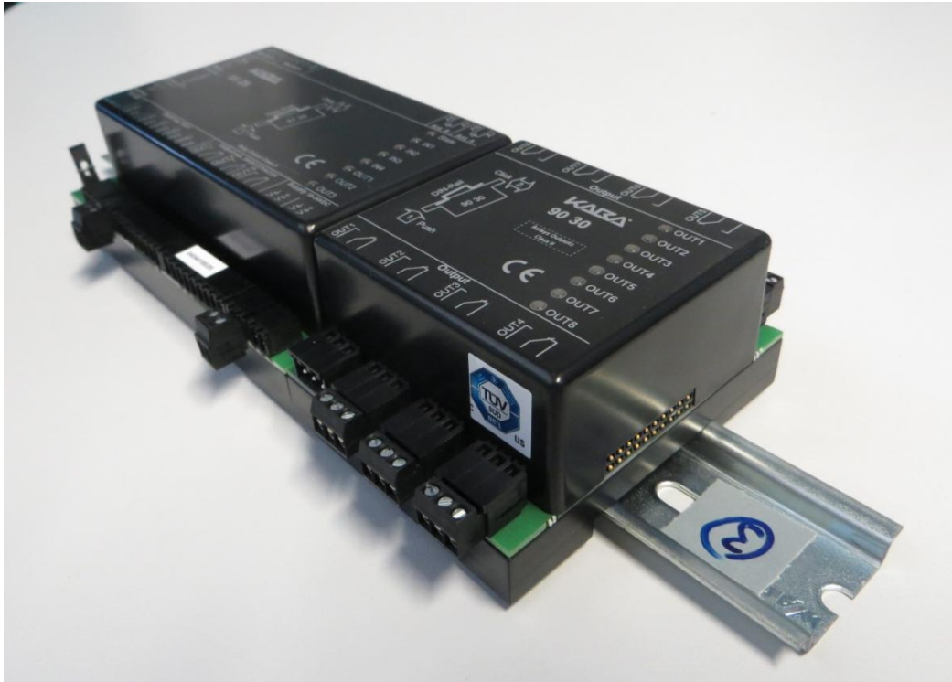
Kaba Remote reader 91 25 & Kaba extension module 90 30
