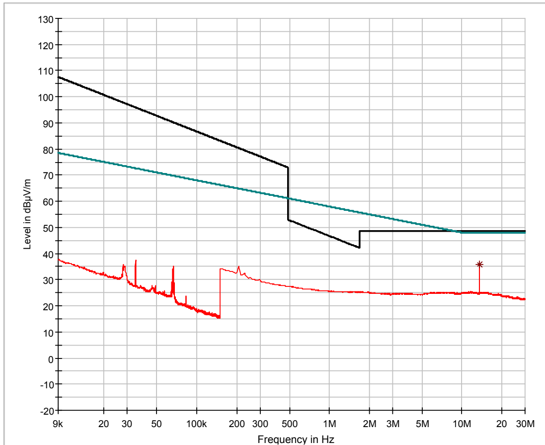
— FCC 15.209 mag (10 m) — EN 300 330 tx mag — Preview Result 1-QPK * Final Result 1-QPK
