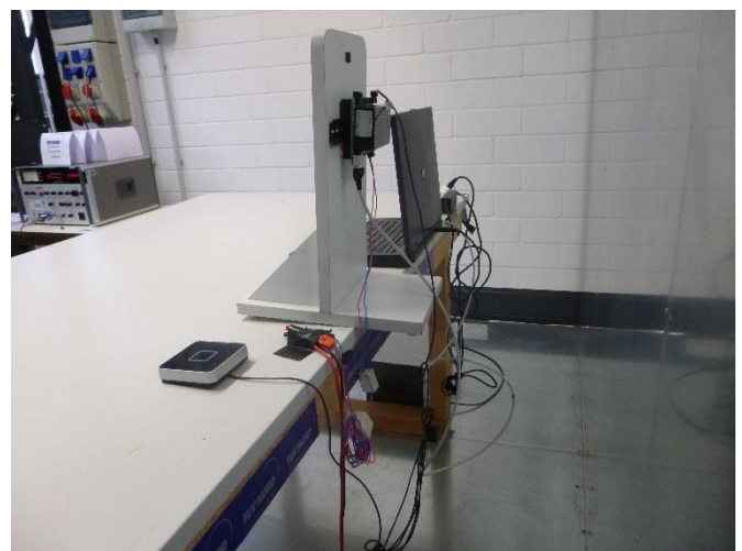
Registration-Unit 9001-BLE
